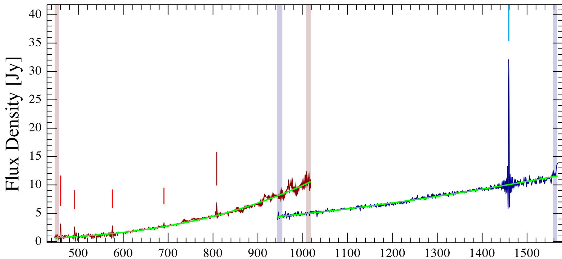
ngc 891 - spire upper pointing-1 Observation ID 1342224766; (6/1)
