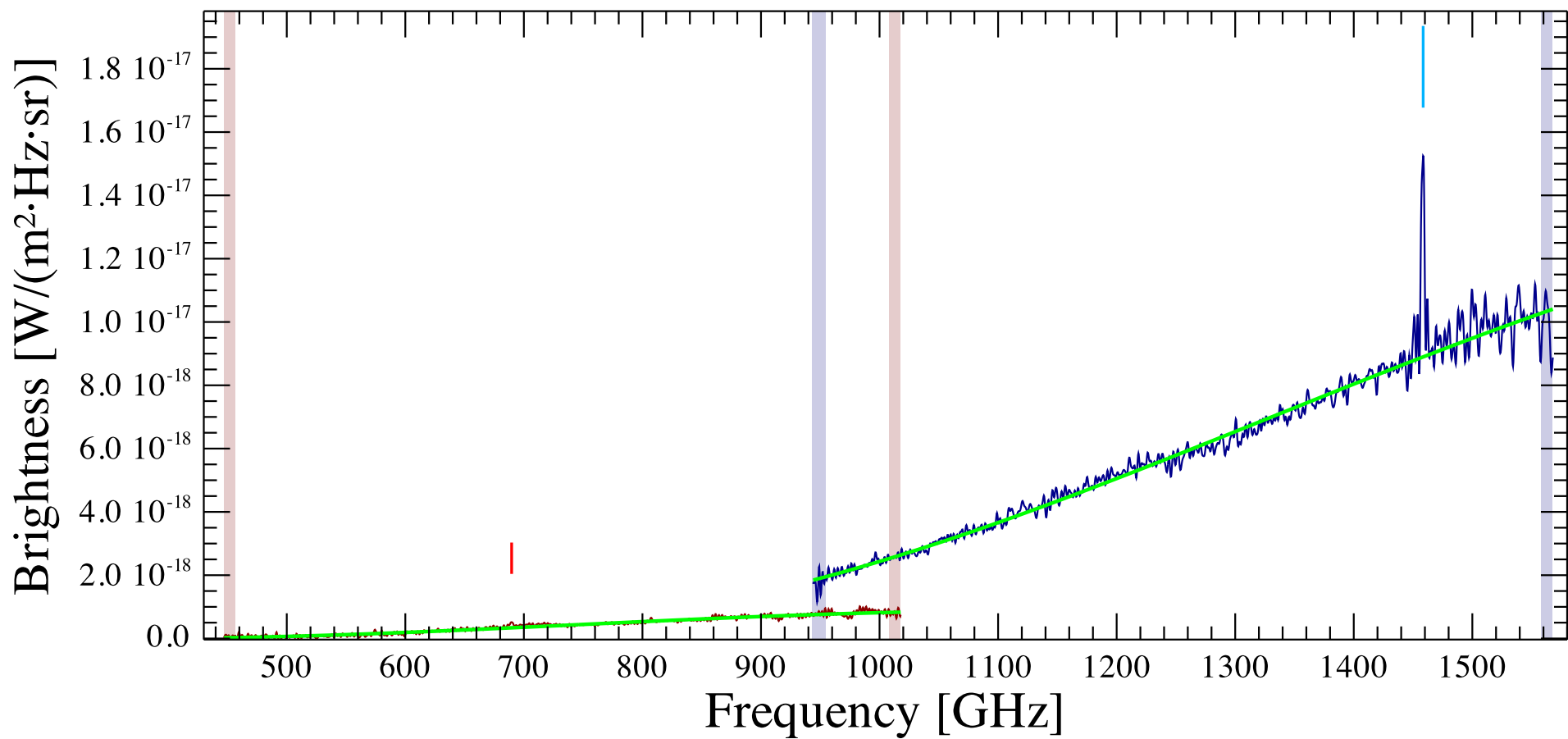
NGC4526 Observation ID 1342224762; (1/1)
