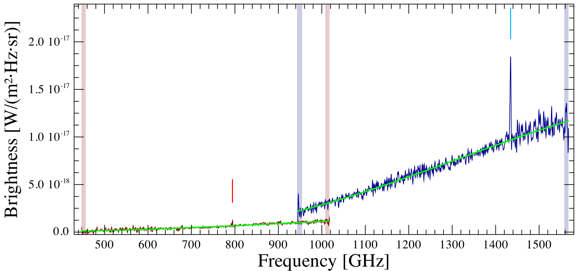
NGC6286a Observation ID 1342221715; (1/1)
