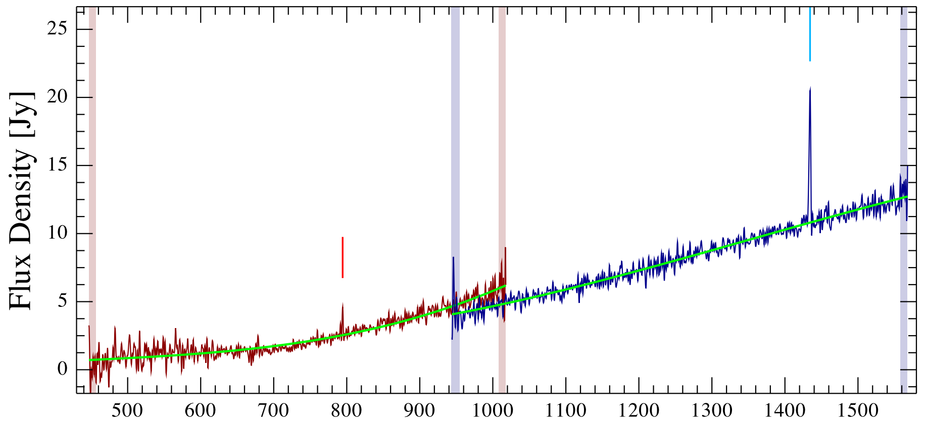
NGC6286a Observation ID 1342221715; (1/1)
