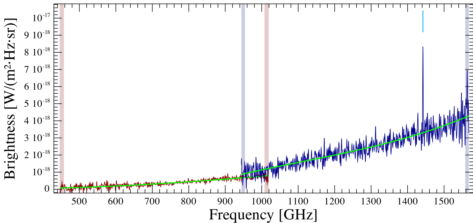
NGC3221 Observation ID 1342221714; (0/1)
