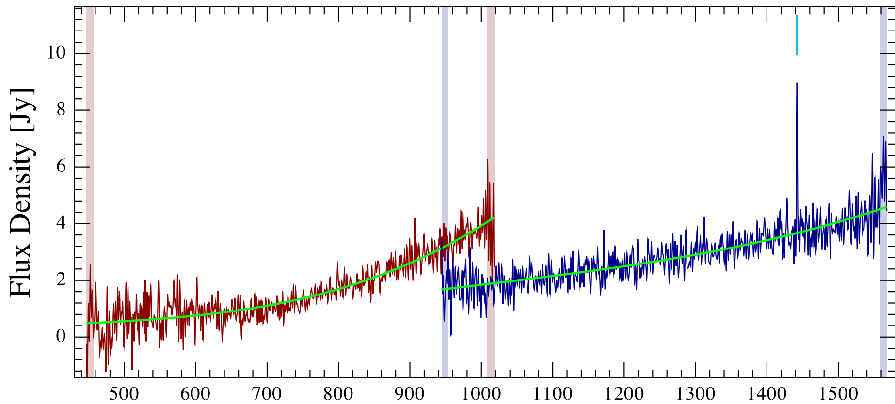
NGC3221 Observation ID 1342221714; (0/1)
