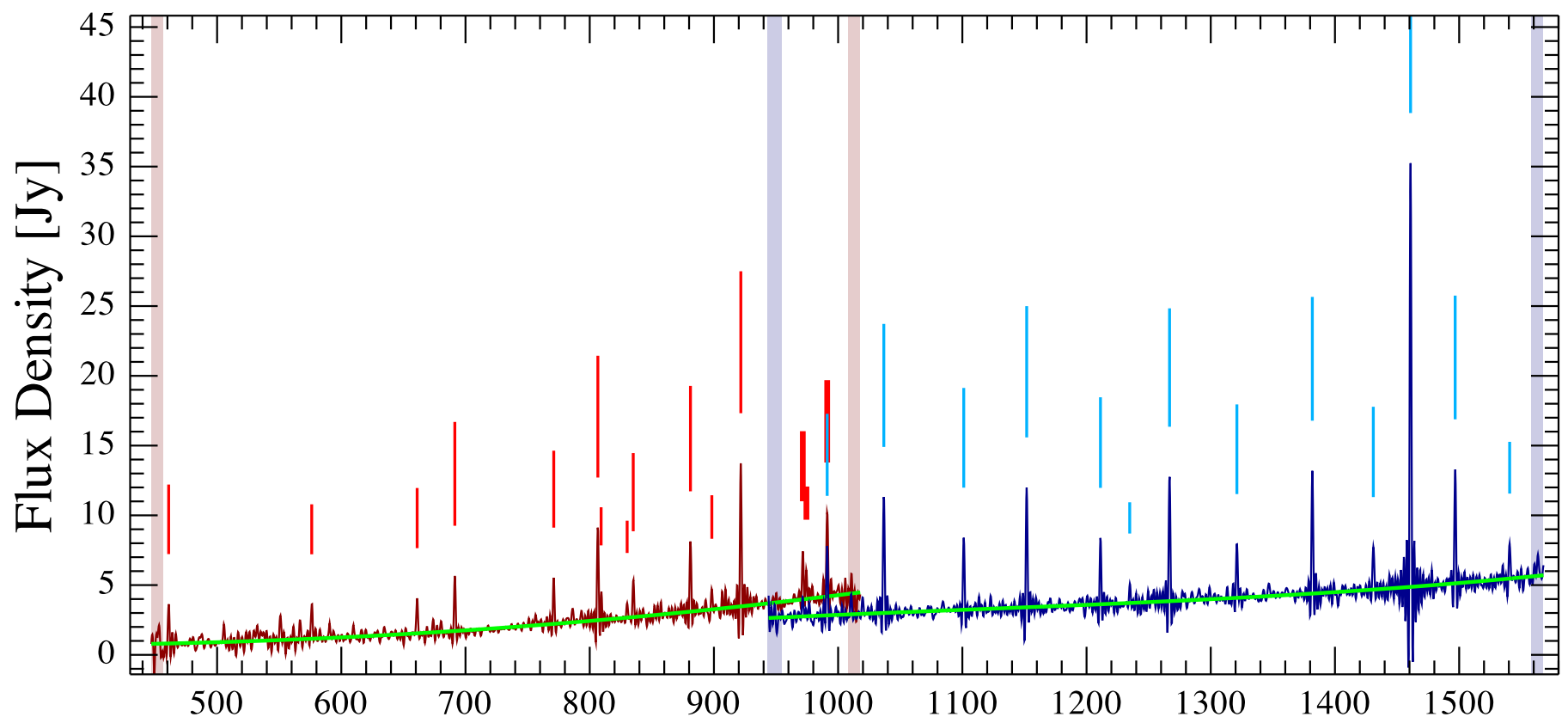
NGC 2440 Observation ID 1342221712; (12/13)
