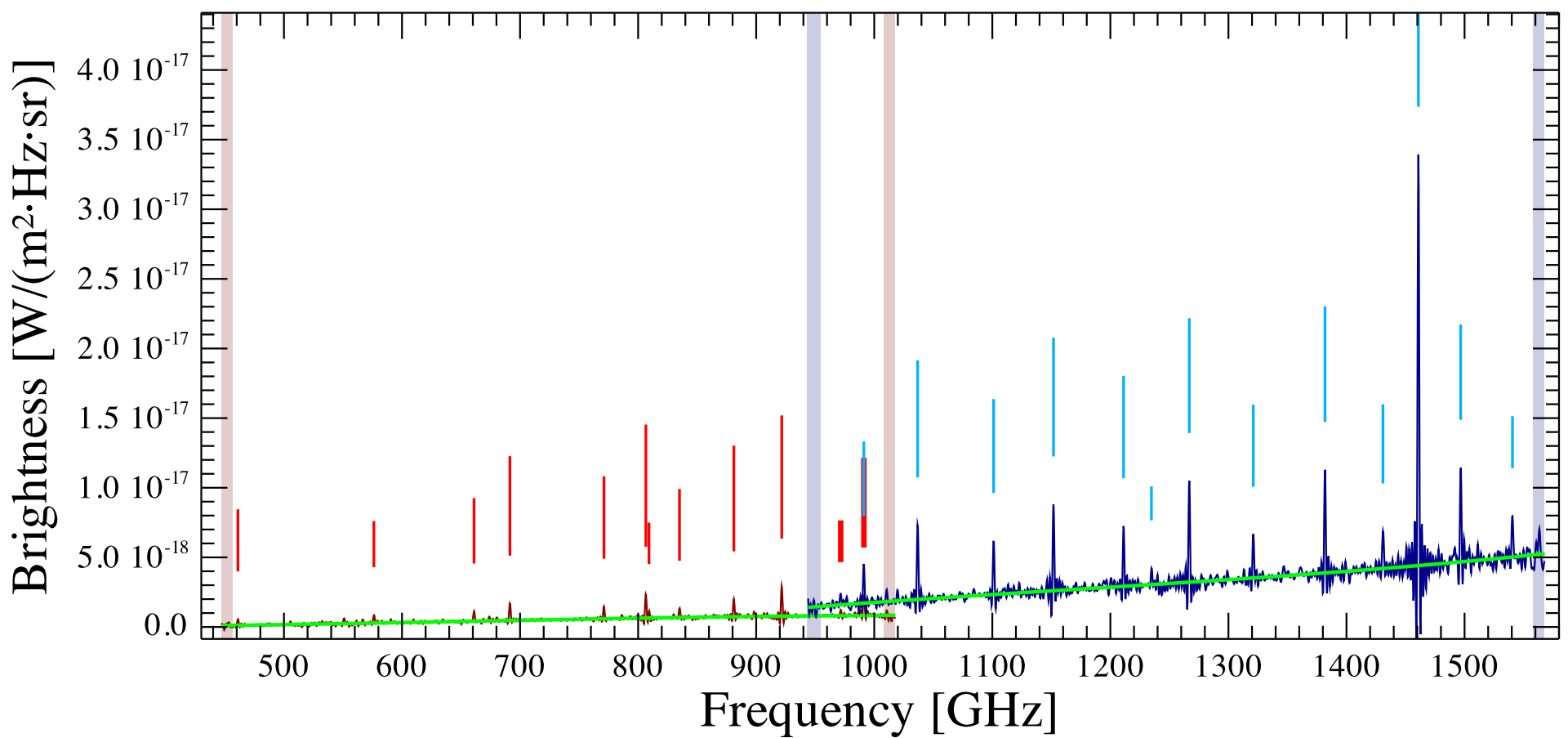
NGC 2440 Observation ID 1342221712; (12/13)
