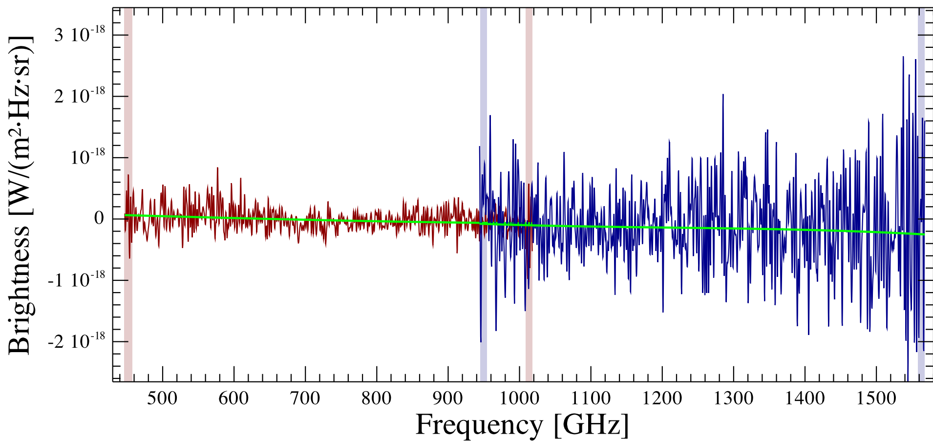
NGC 6826 OFF Observation ID 1342221686; (0/0)
