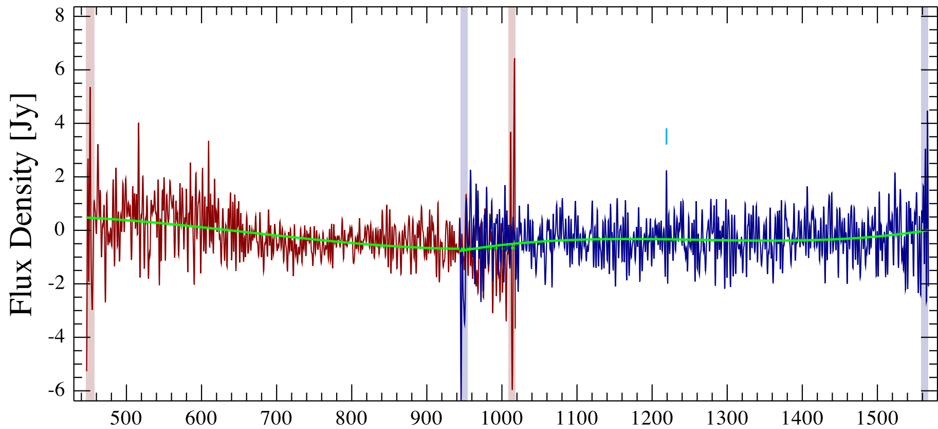
NGC 7009 OFF Observation ID 1342221680; (0/1)
