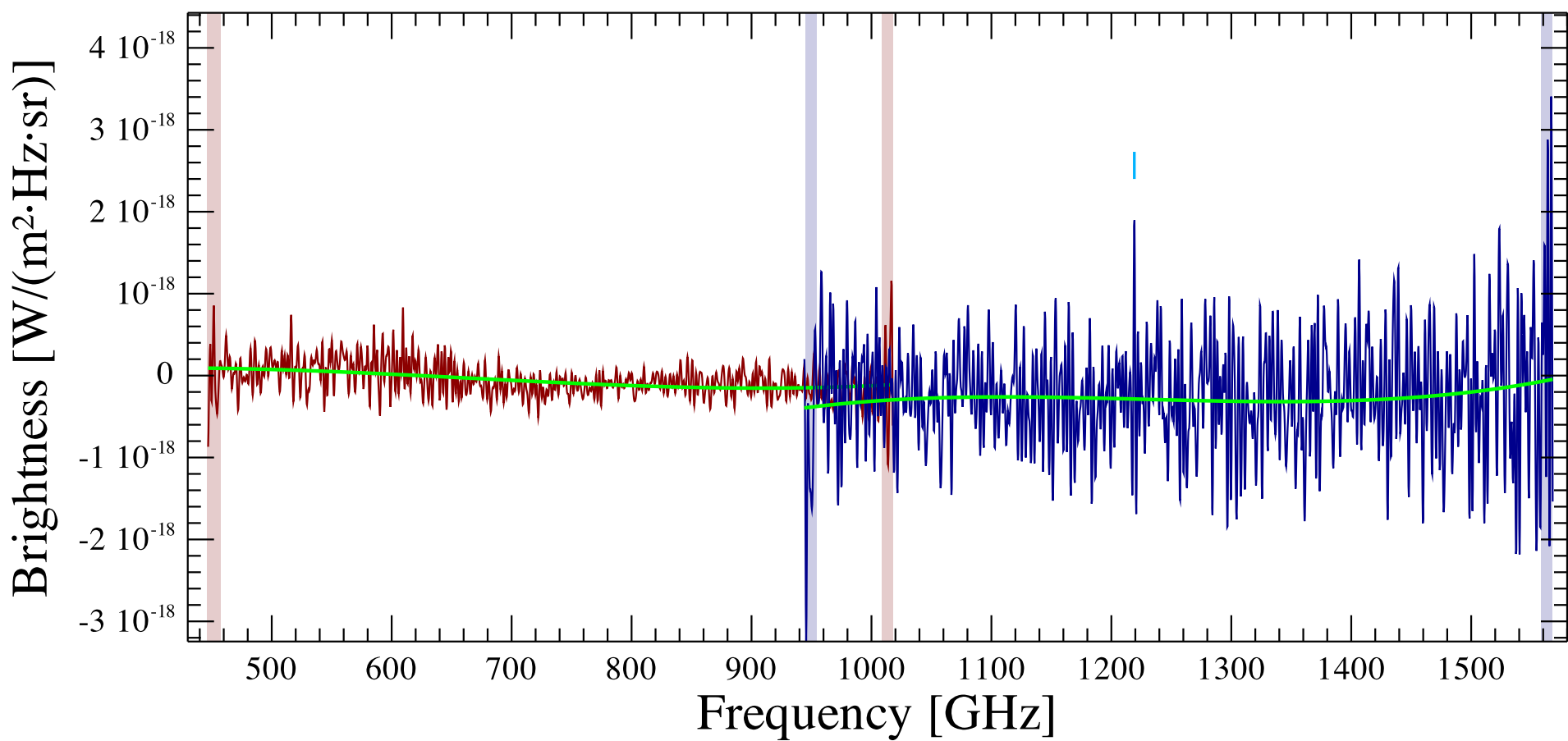
NGC 7009 OFF Observation ID 1342221680; (0/1)
