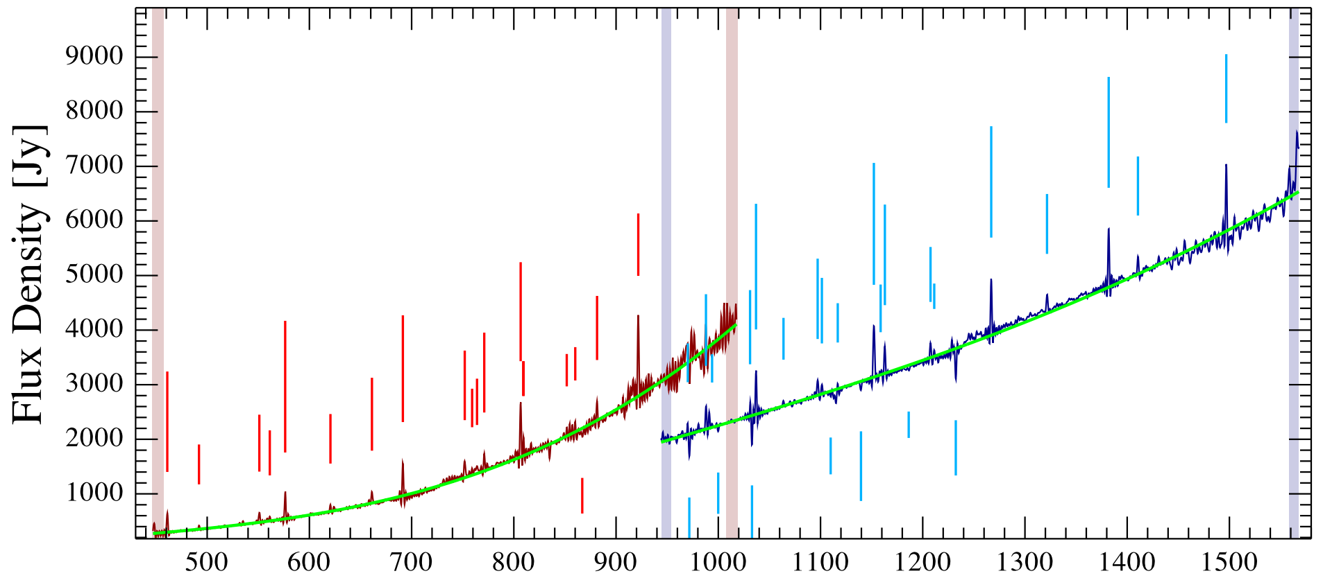
W49N Observation ID 1342219567; (16/15)
