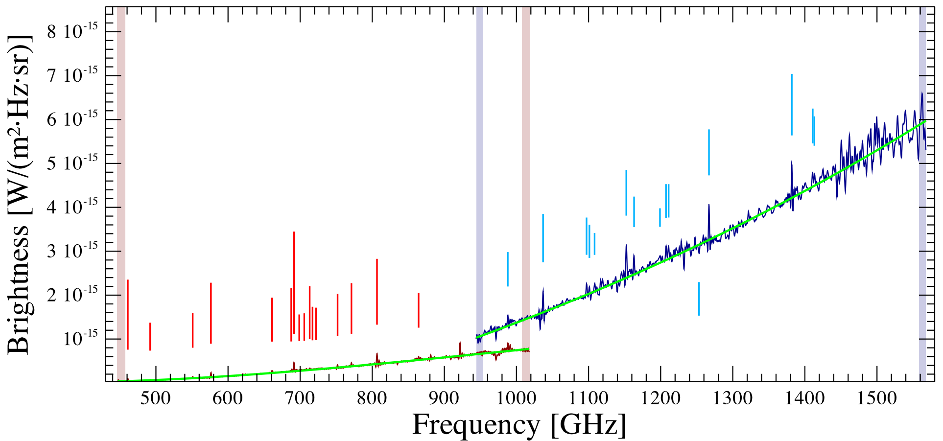
W49N Observation ID 1342219567; (16/15)
