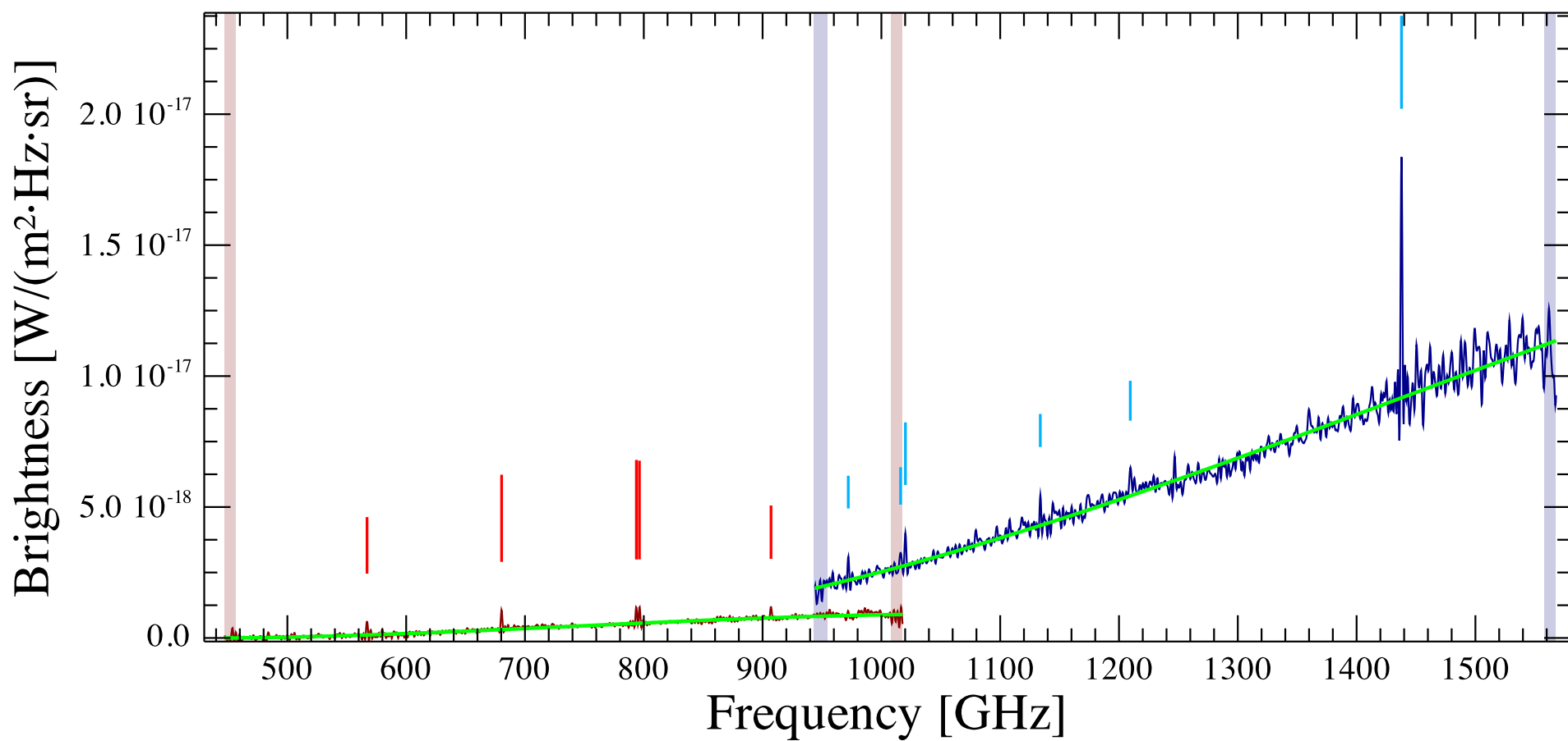
NGC7130 Observation ID 1342219565; (5/6)
