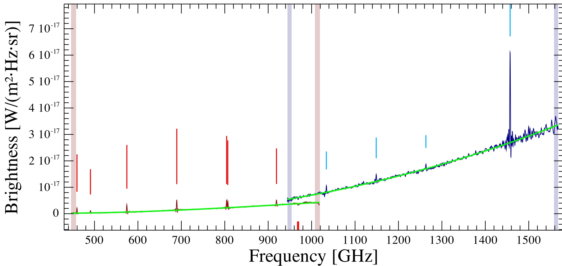
NGC2146-SE Observation ID 1342219555; (8/4)
