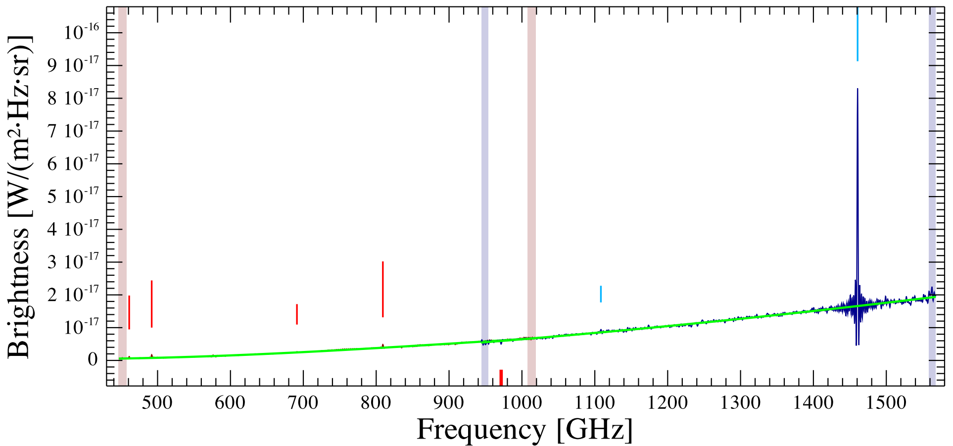
los_26.46+0.09 Observation ID 1342216897; (5/2)
