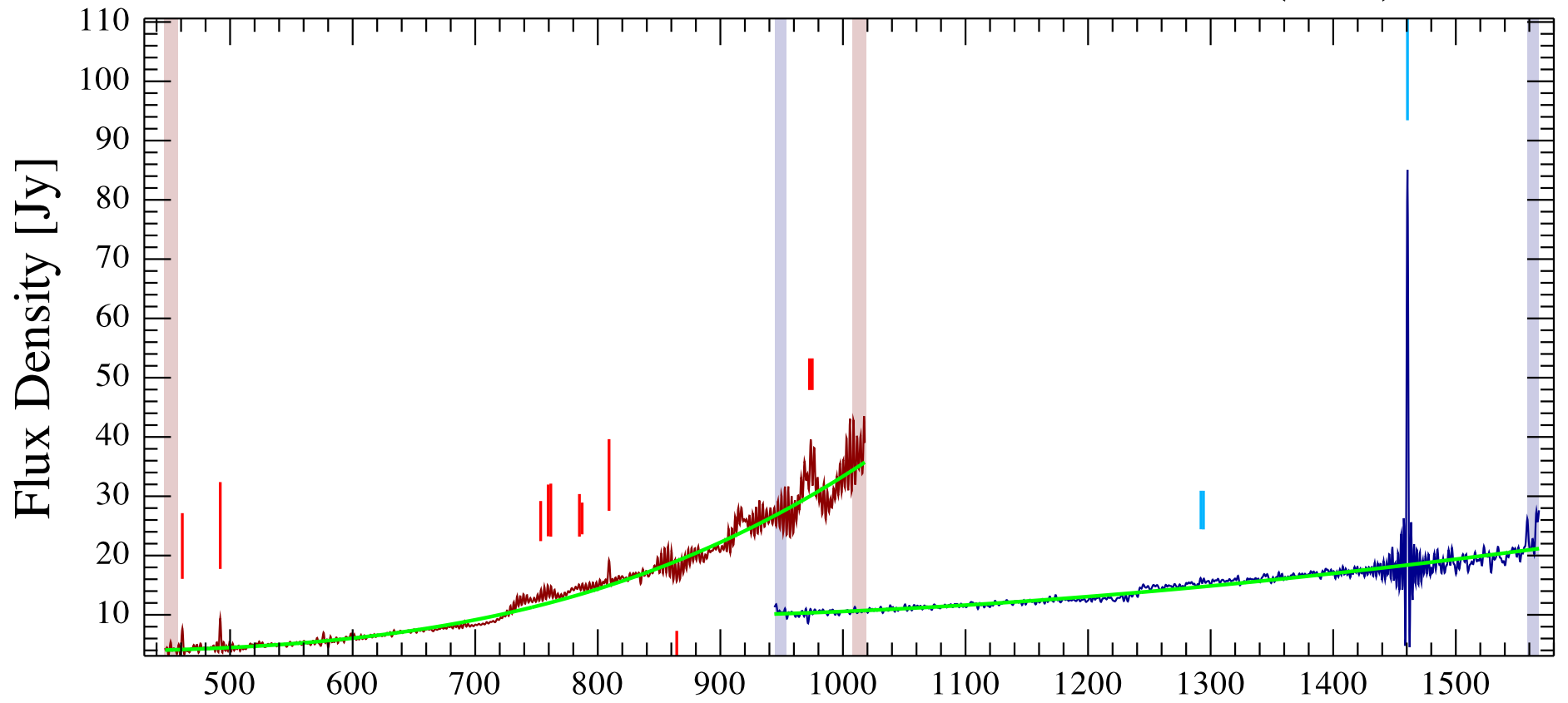
los_26.46+0.09 Observation ID 1342216897; (5/2)
