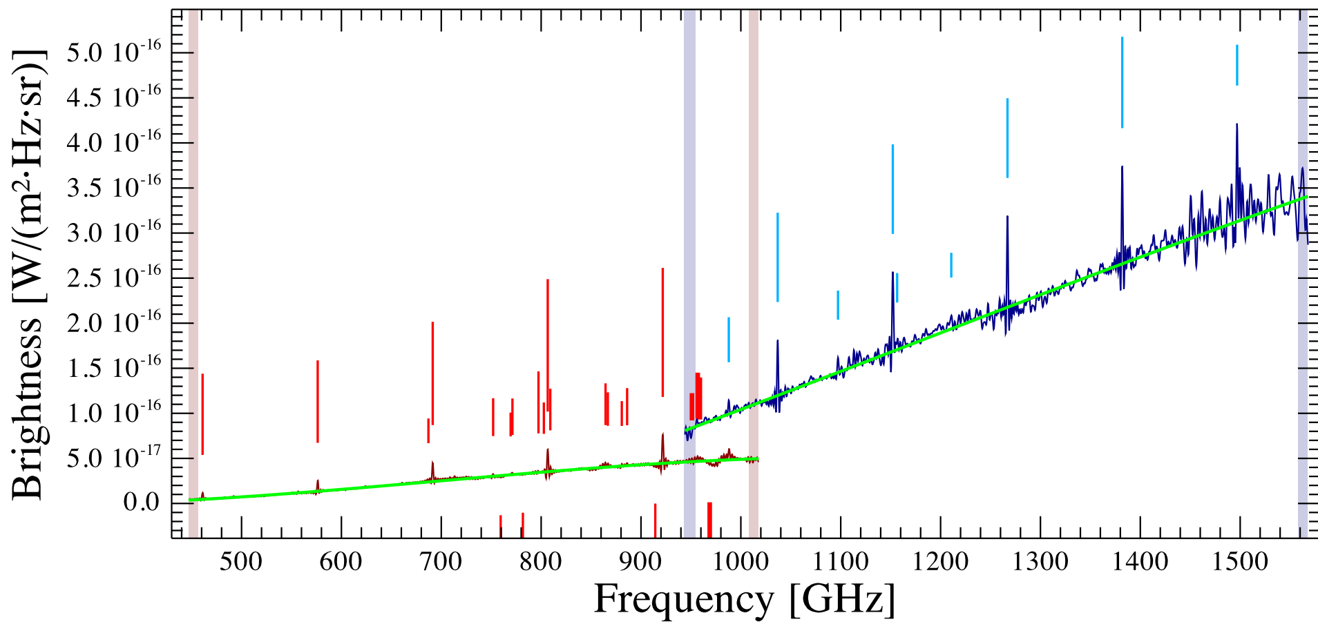
SERPENS_MM1 Observation ID 1342216893; (23/9)
