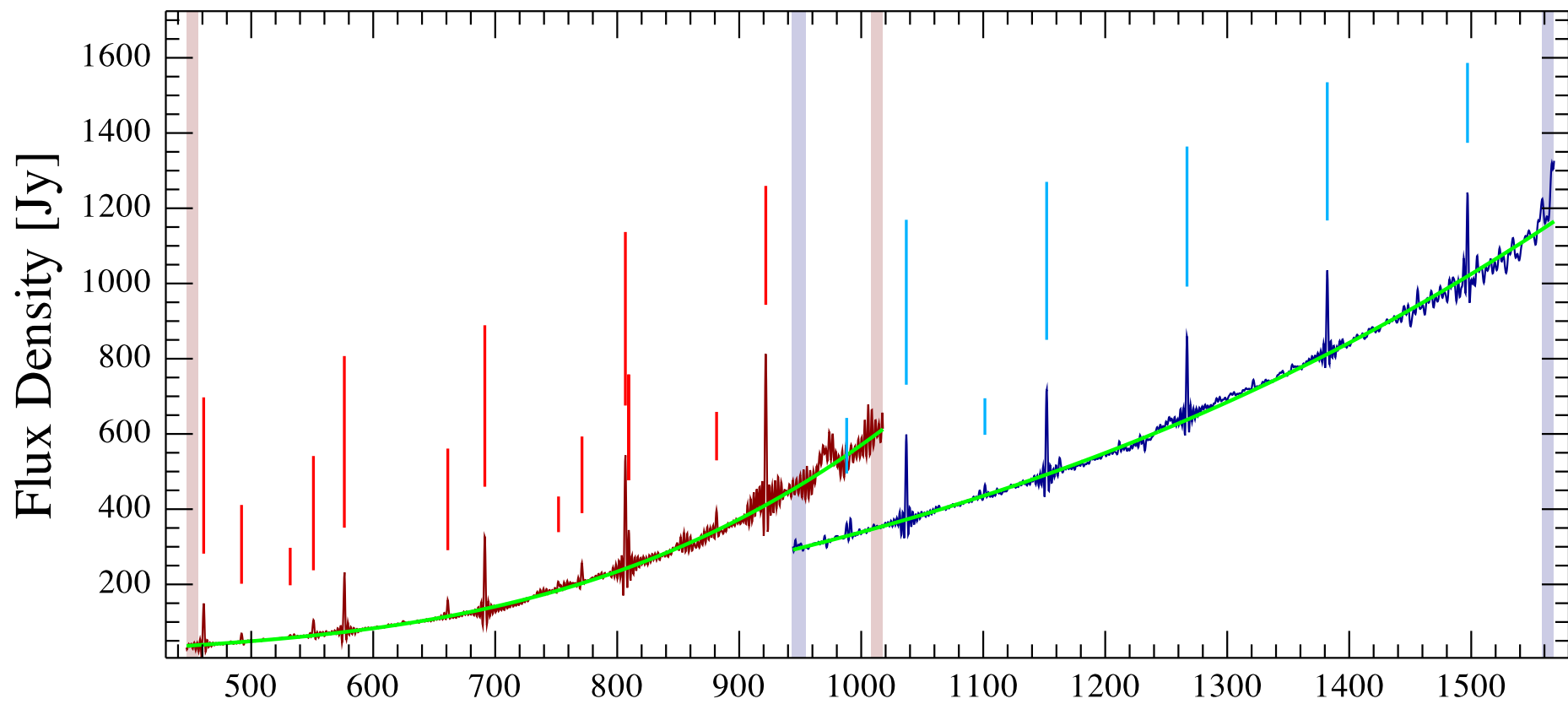
AFGL 2591 Observation ID 1342216892; (25/12)
