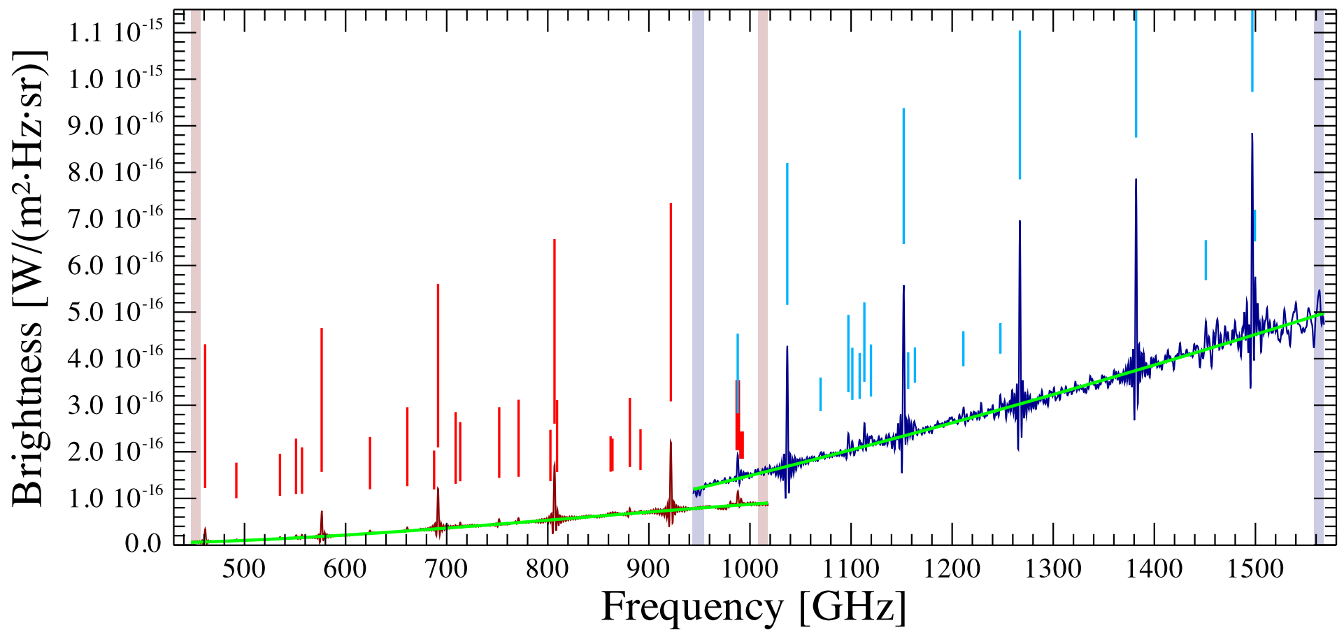
NGC_2071 Observation ID 1342216883; (25/18)
