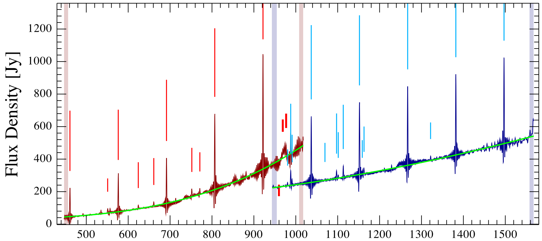
NGC_2071 Observation ID 1342216883; (25/18)
