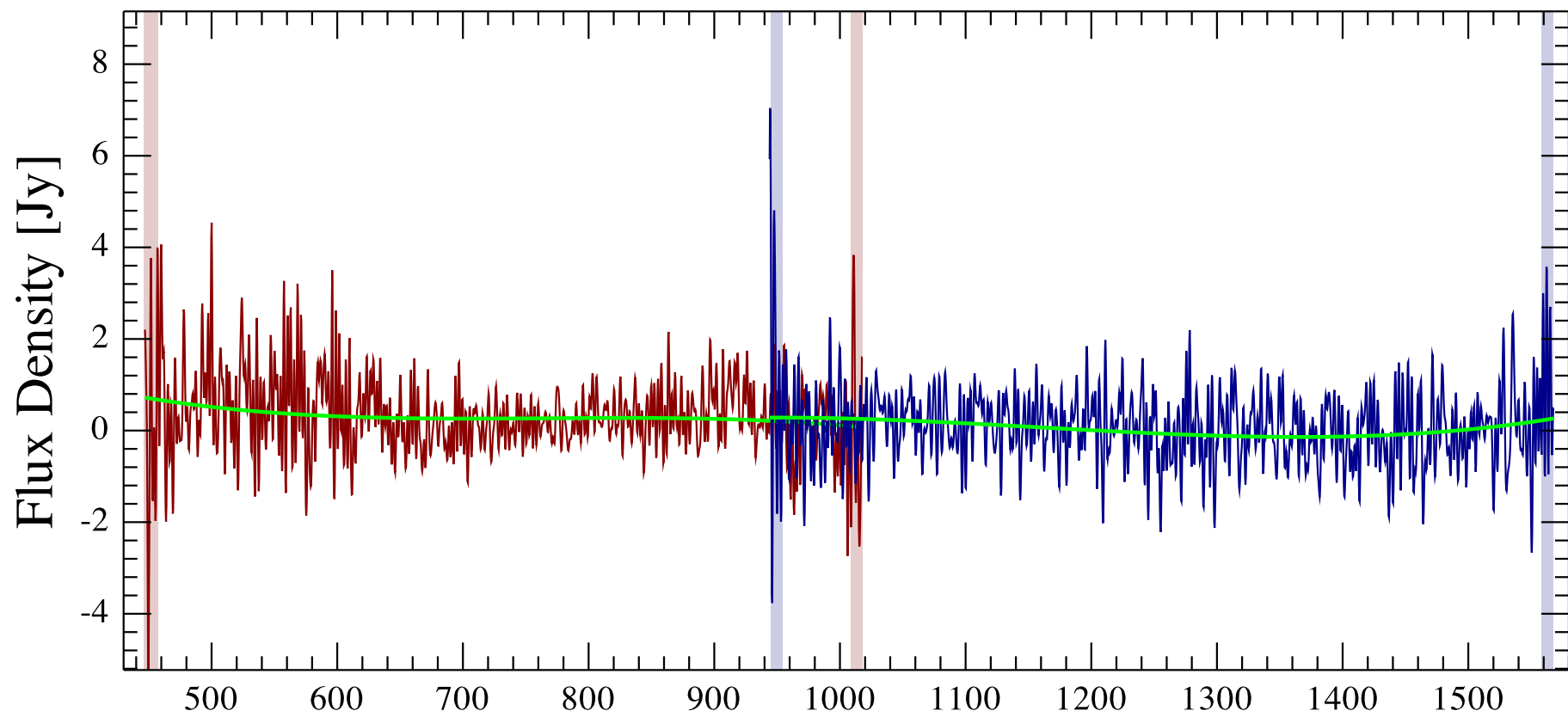
L1489-IRS_off Observation ID 1342214856; (0/0)
