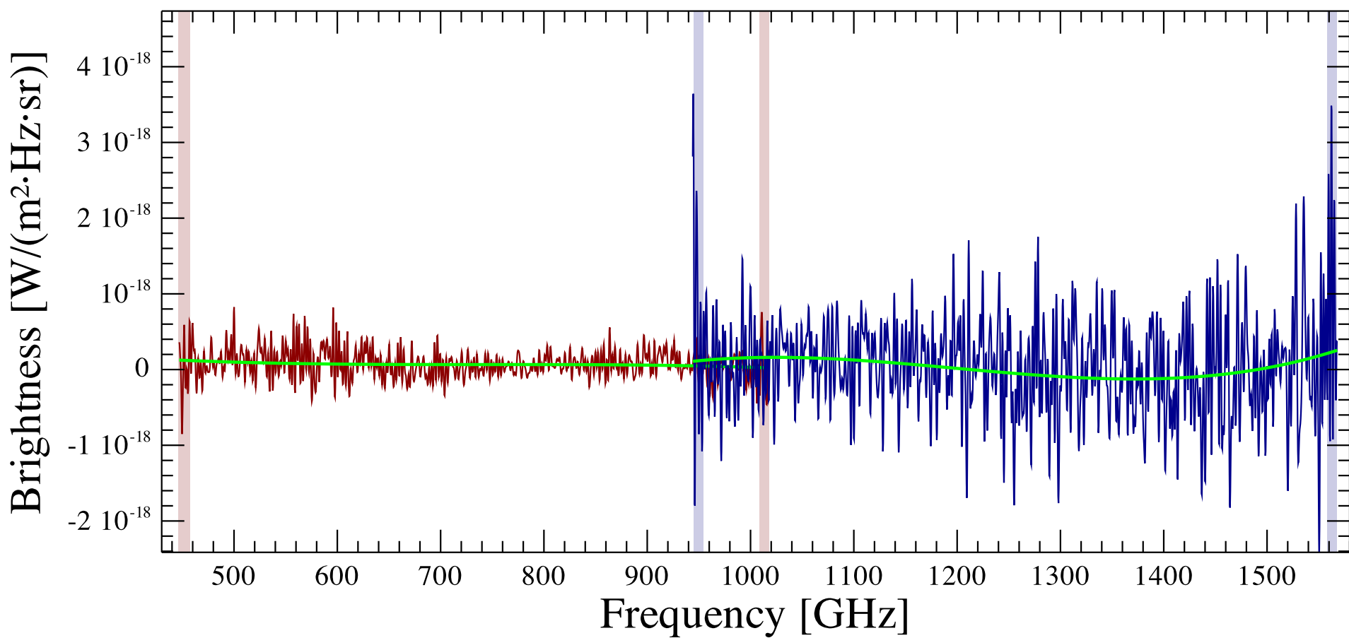
L1489-IRS_off Observation ID 1342214856; (0/0)
