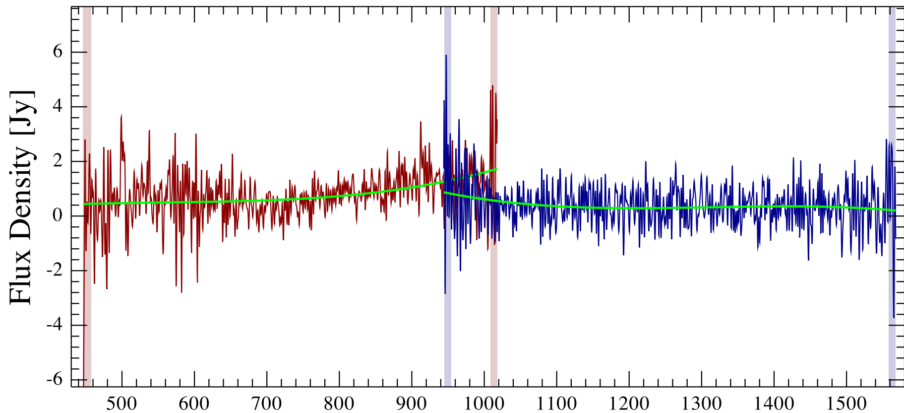
IRAx04191_off Observation ID 1342214852; (0/0)
