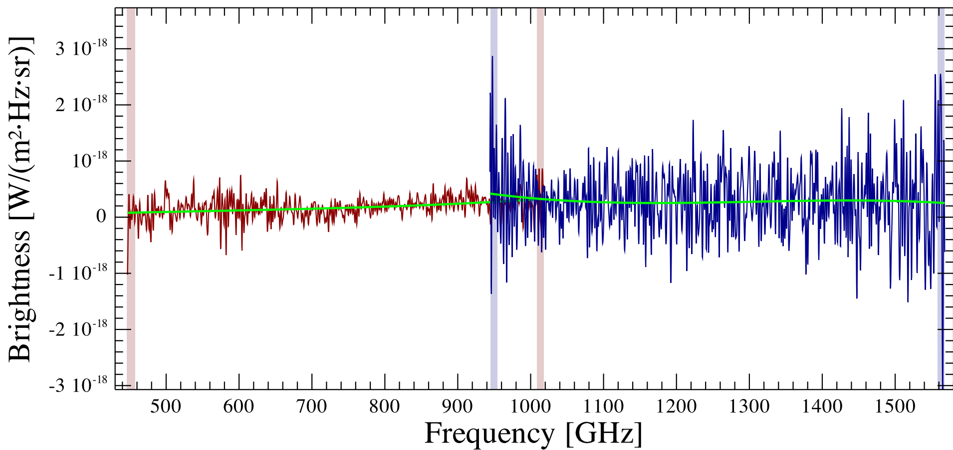
IRAx04191_off Observation ID 1342214852; (0/0)
