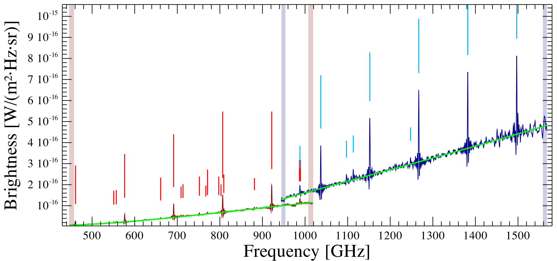
OMC2_FIR4 Observation ID 1342214847; (18/9)
