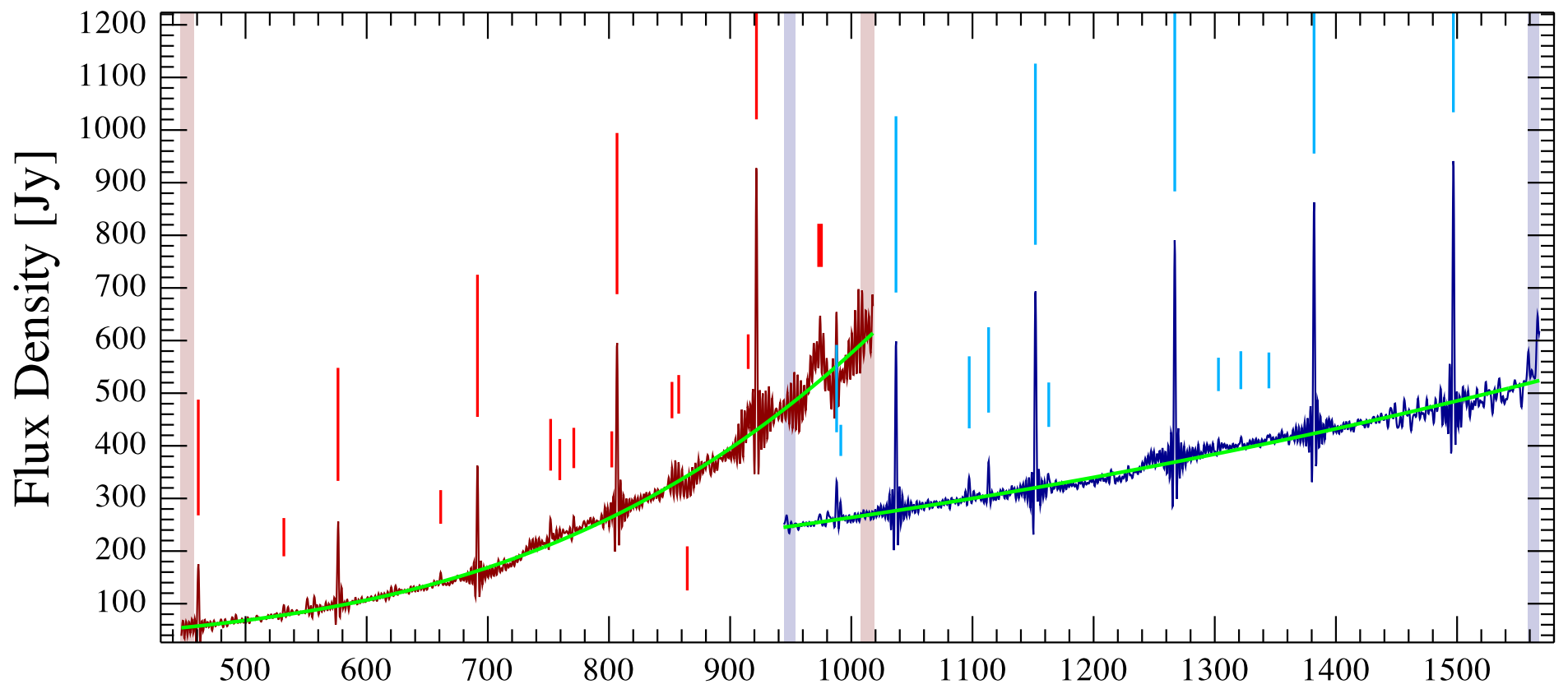
OMC2_FIR4 Observation ID 1342214847; (18/9)
