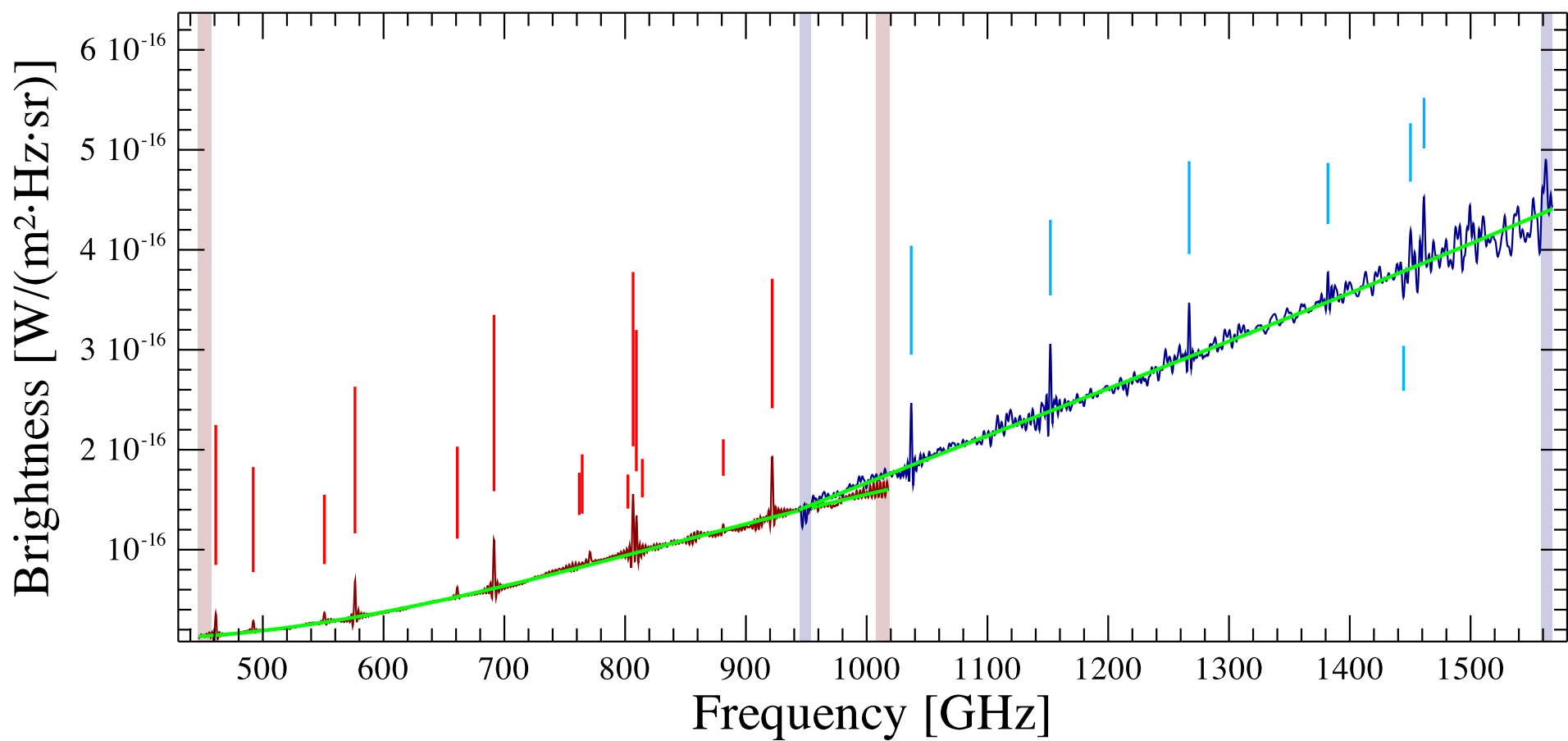
NGC6334_int Observation ID 1342214828; (14/7)
