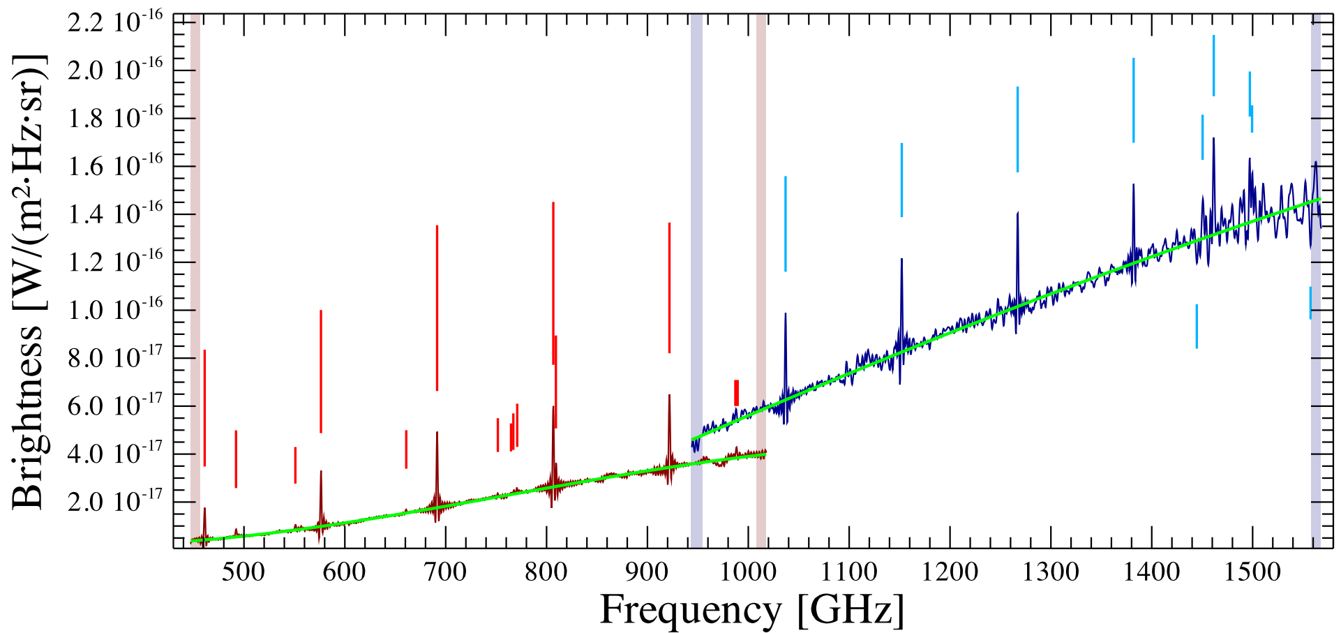
RCW120-38 Observation ID 1342214825; (14/10)
