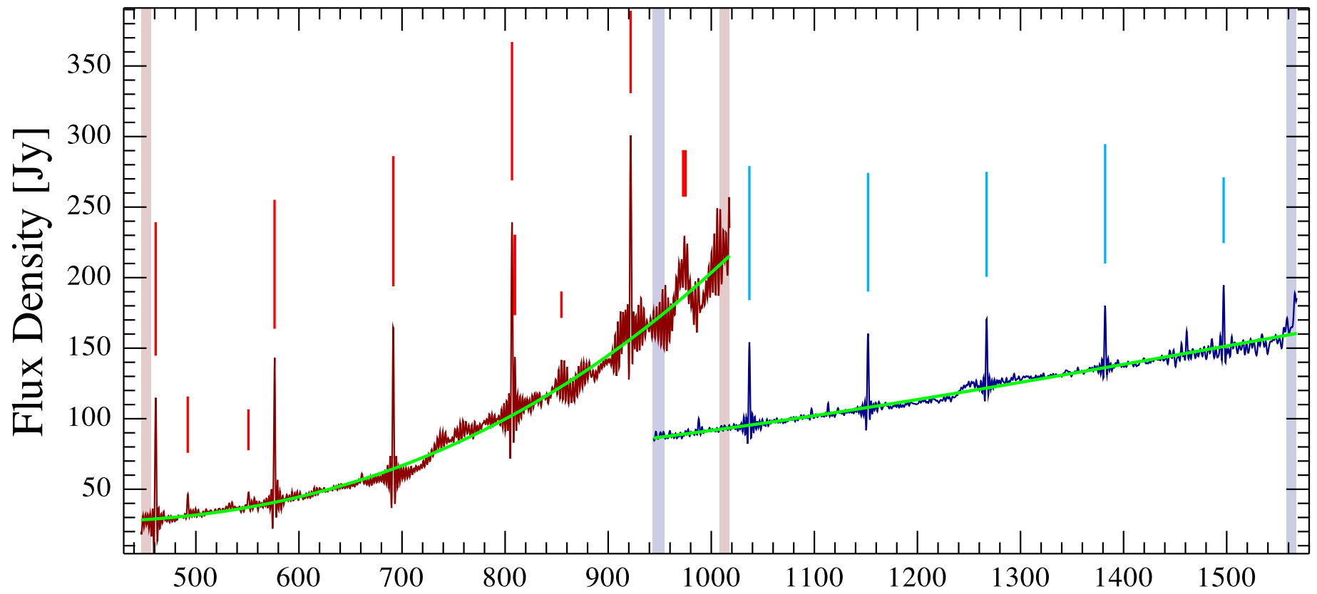
RCW120-38 Observation ID 1342214825; (14/10)
