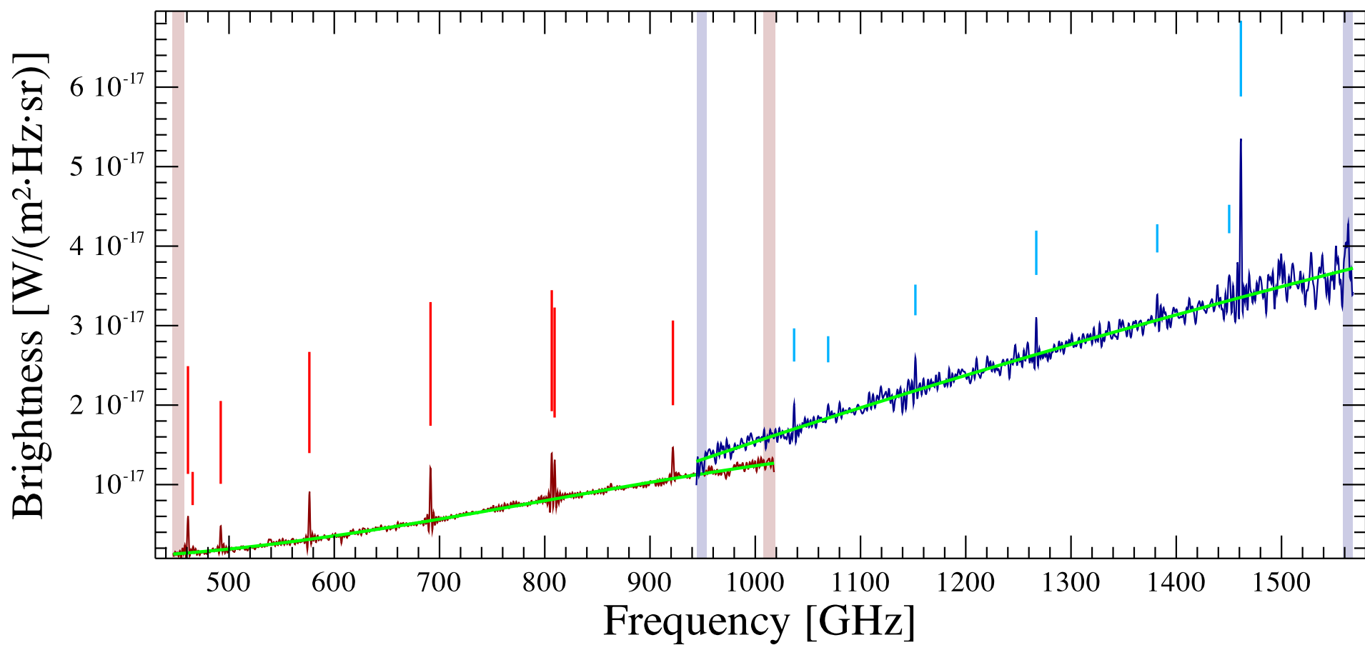
RCW120-76-1 Observation ID 1342214824; (8/7)
