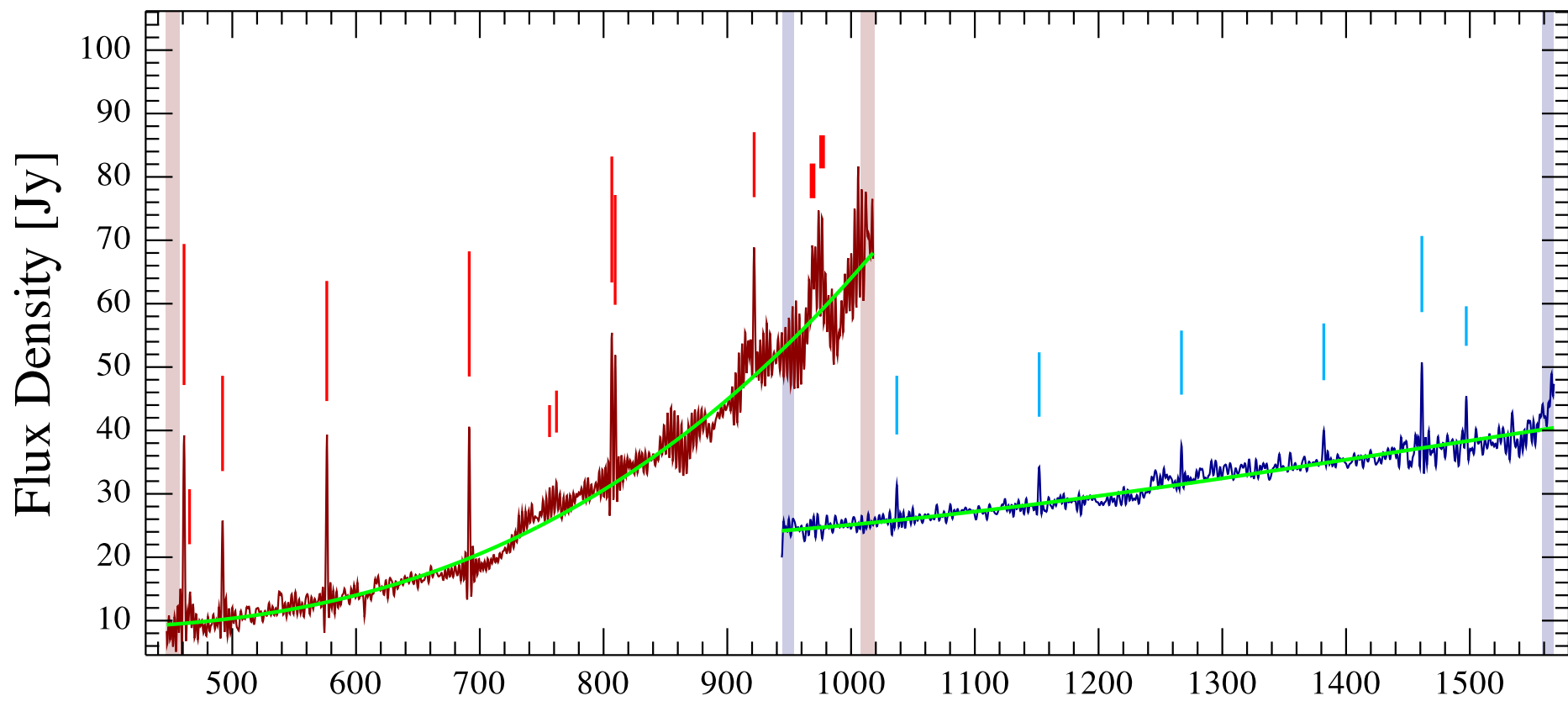
RCW120-76-1 Observation ID 1342214824; (8/7)
