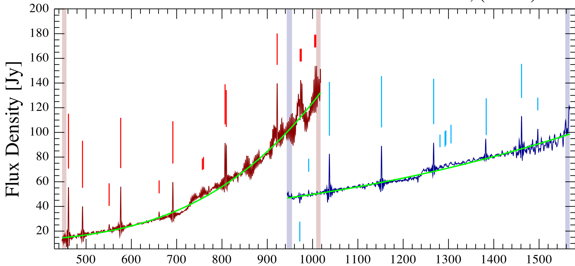
Iras16132cond1-1 Observation ID 1342214820; (11/6)
