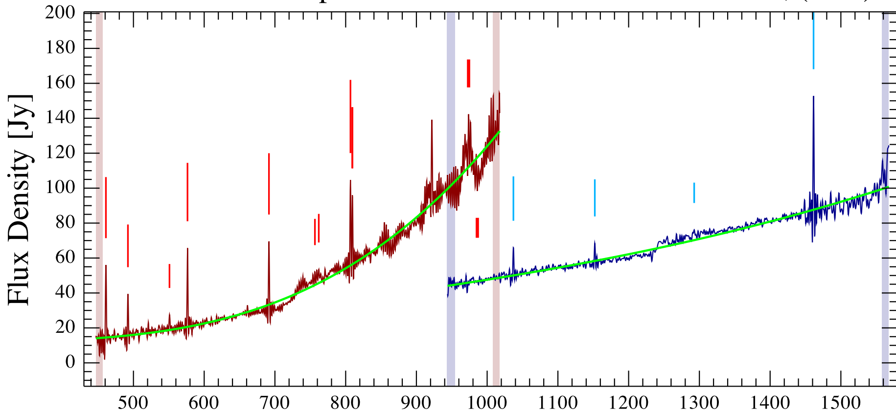
Iras16132cond0spectro-1 Observation ID 1342214819; (11/4)
