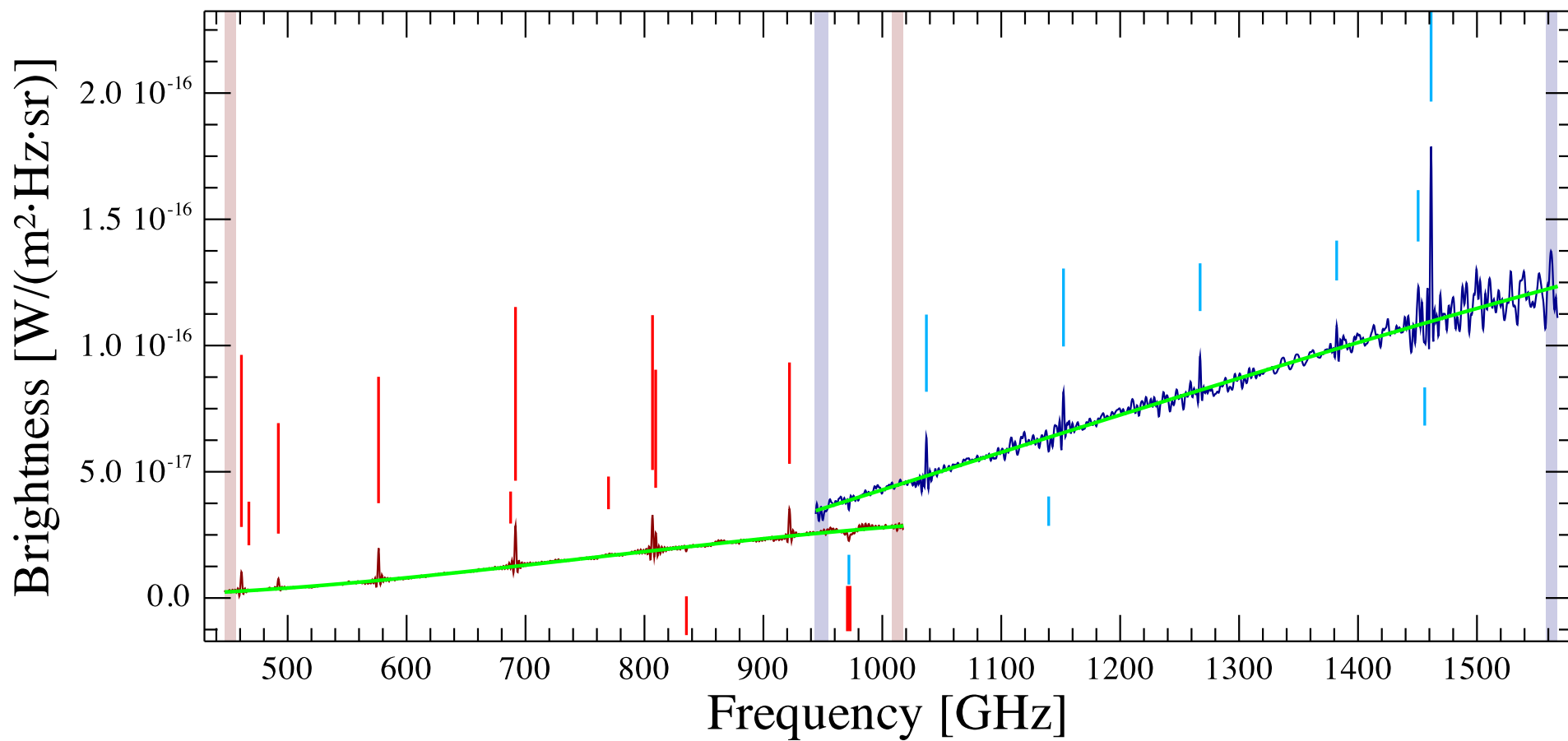
Iras16132maser2-1 Observation ID 1342214817; (12/9)
