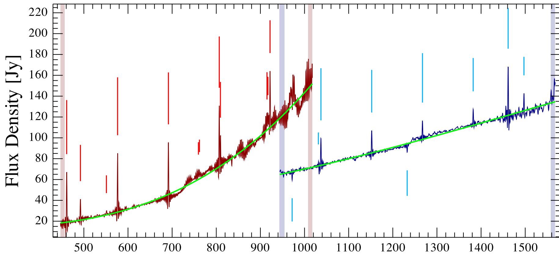
Iras16132maser2-1 Observation ID 1342214817; (12/9)
