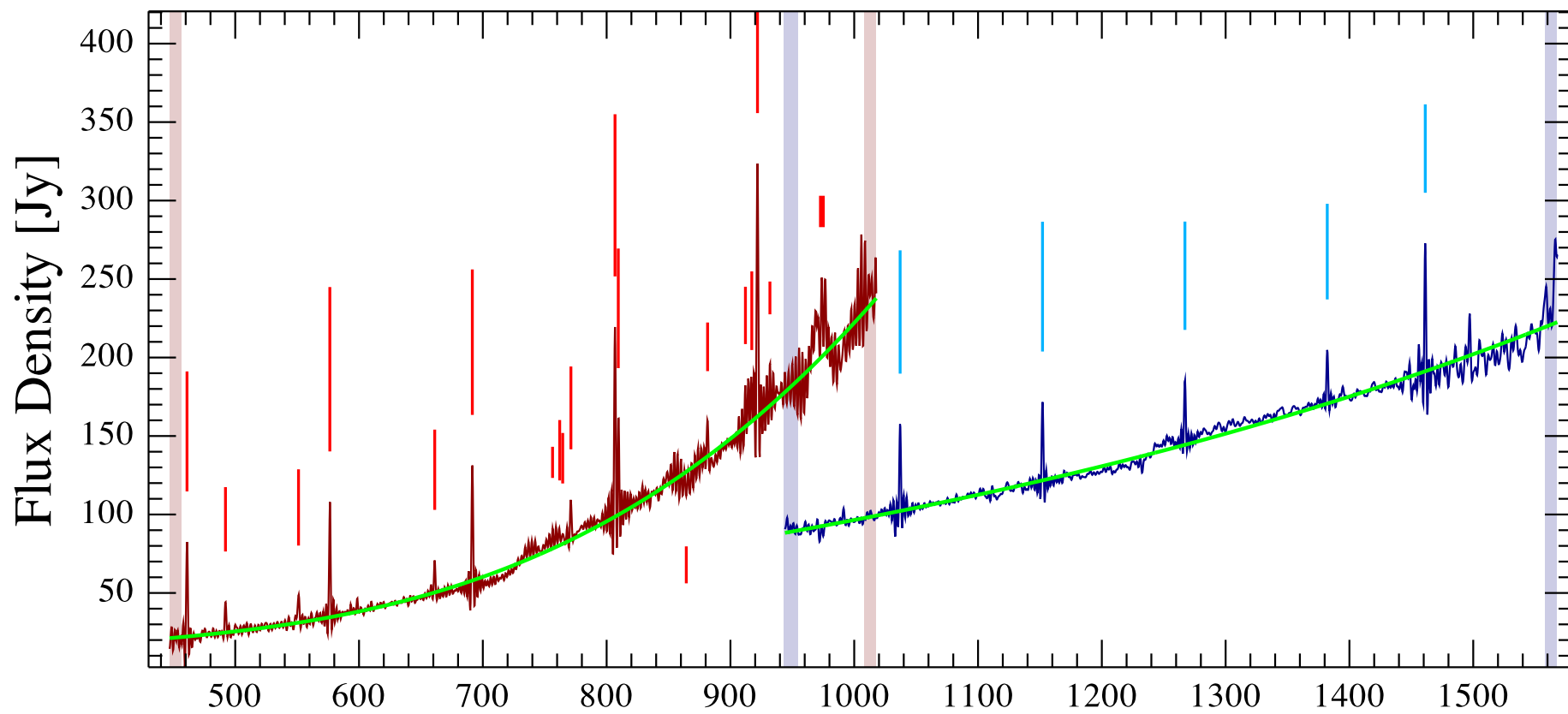
Iras16132spectro-1 Observation ID 1342214816; (13/6)
