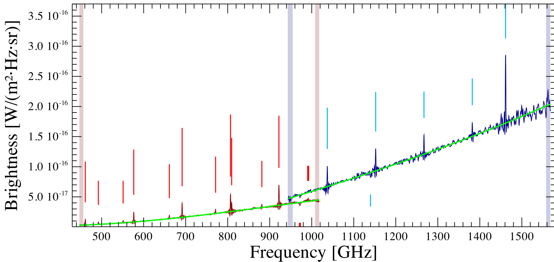
Iras16132spectro-1 Observation ID 1342214816; (13/6)
