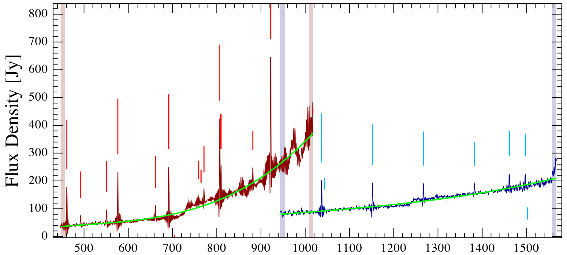
G327 Observation ID 1342214815; (13/7)
