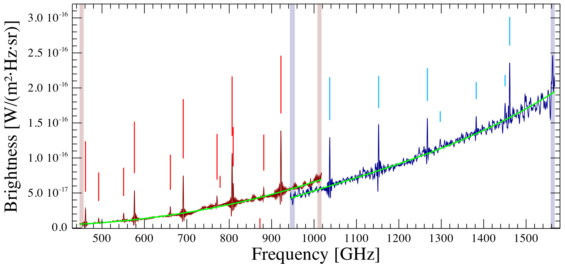
G327 Observation ID 1342214815; (13/7)
