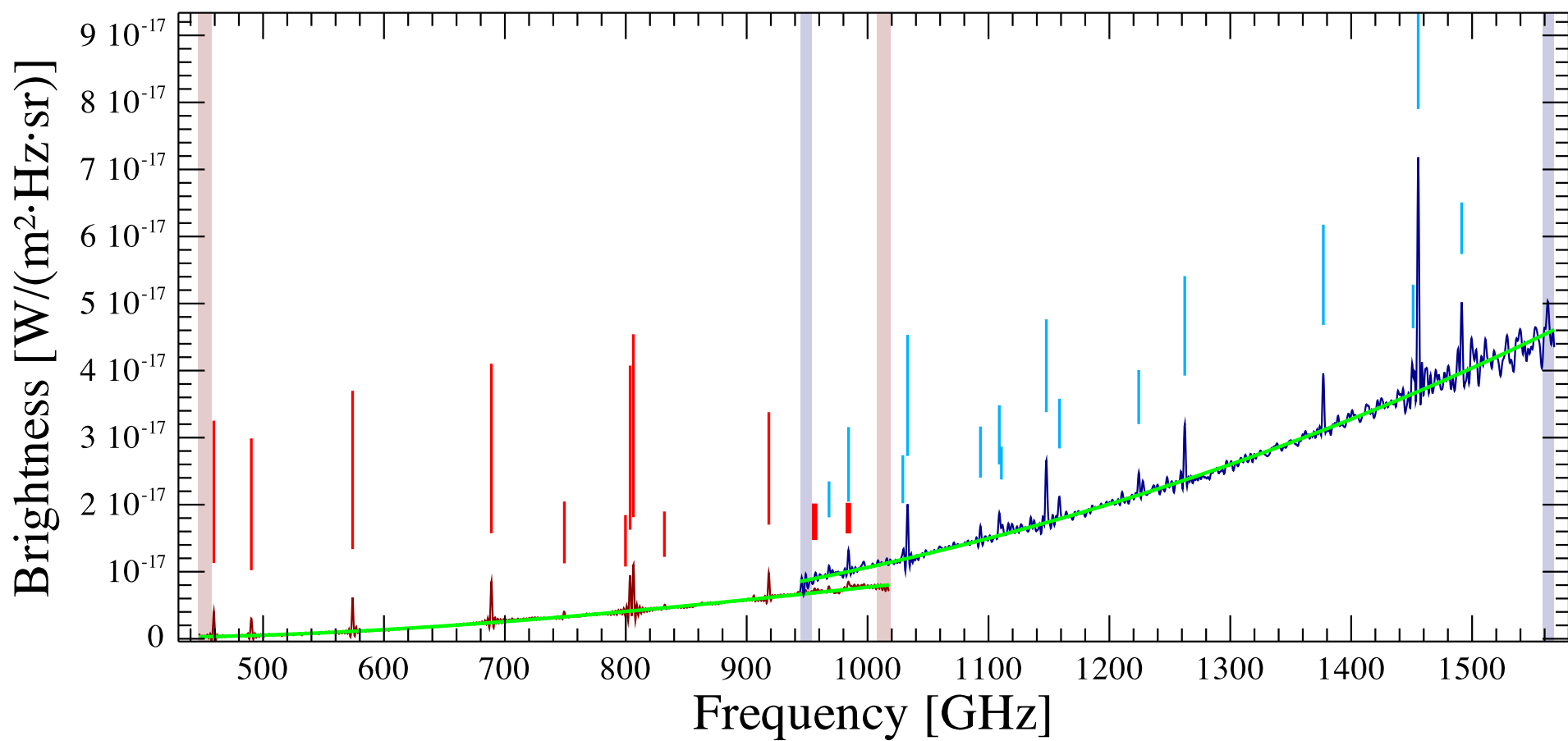
ngc1068 Observation ID 1342213445; (12/15)
