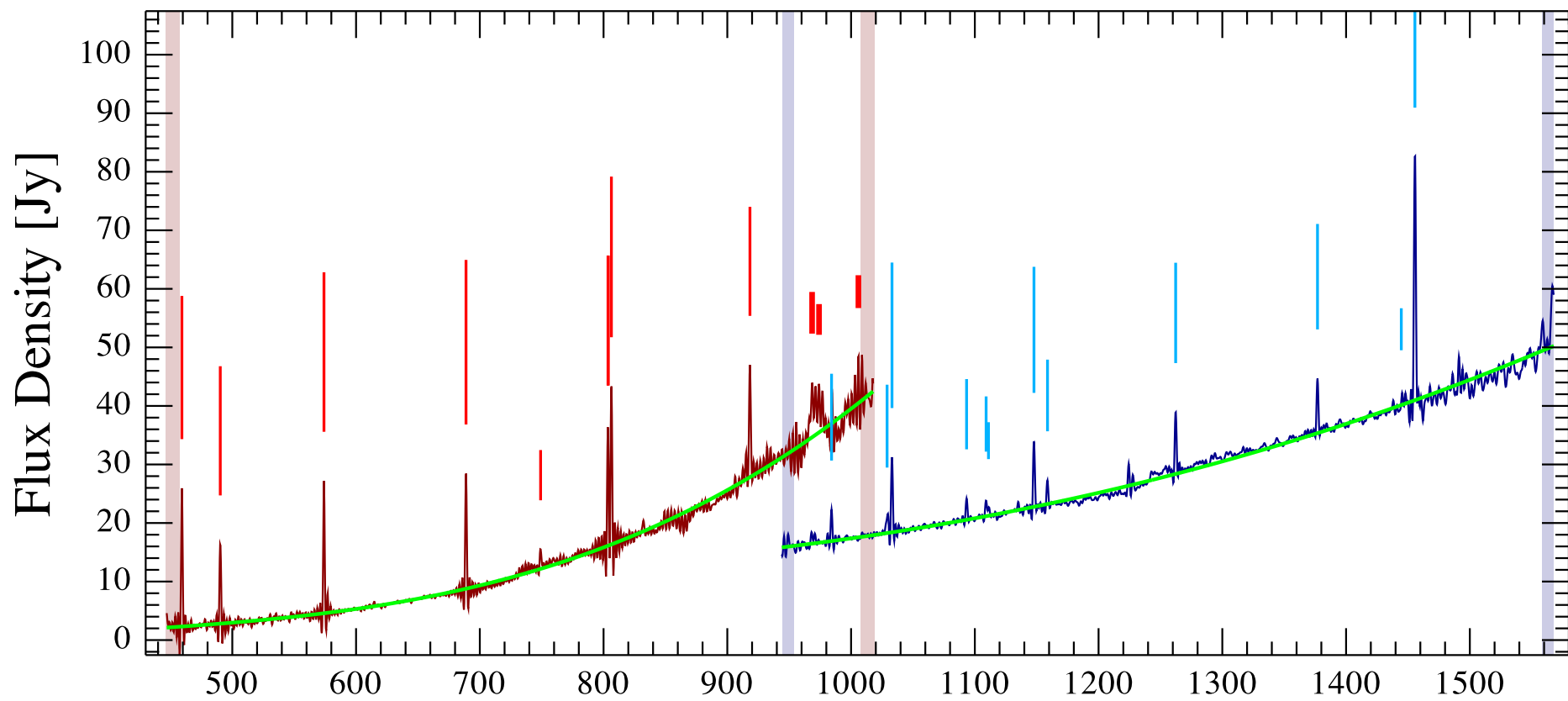
ngc1068 Observation ID 1342213445; (12/15)
