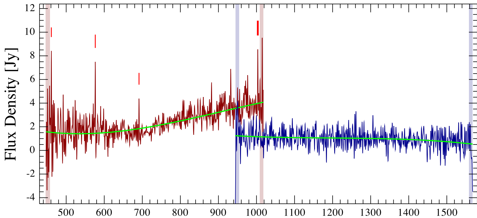
N1333-IRAS4_off Observation ID 1342213375; (3/0)
