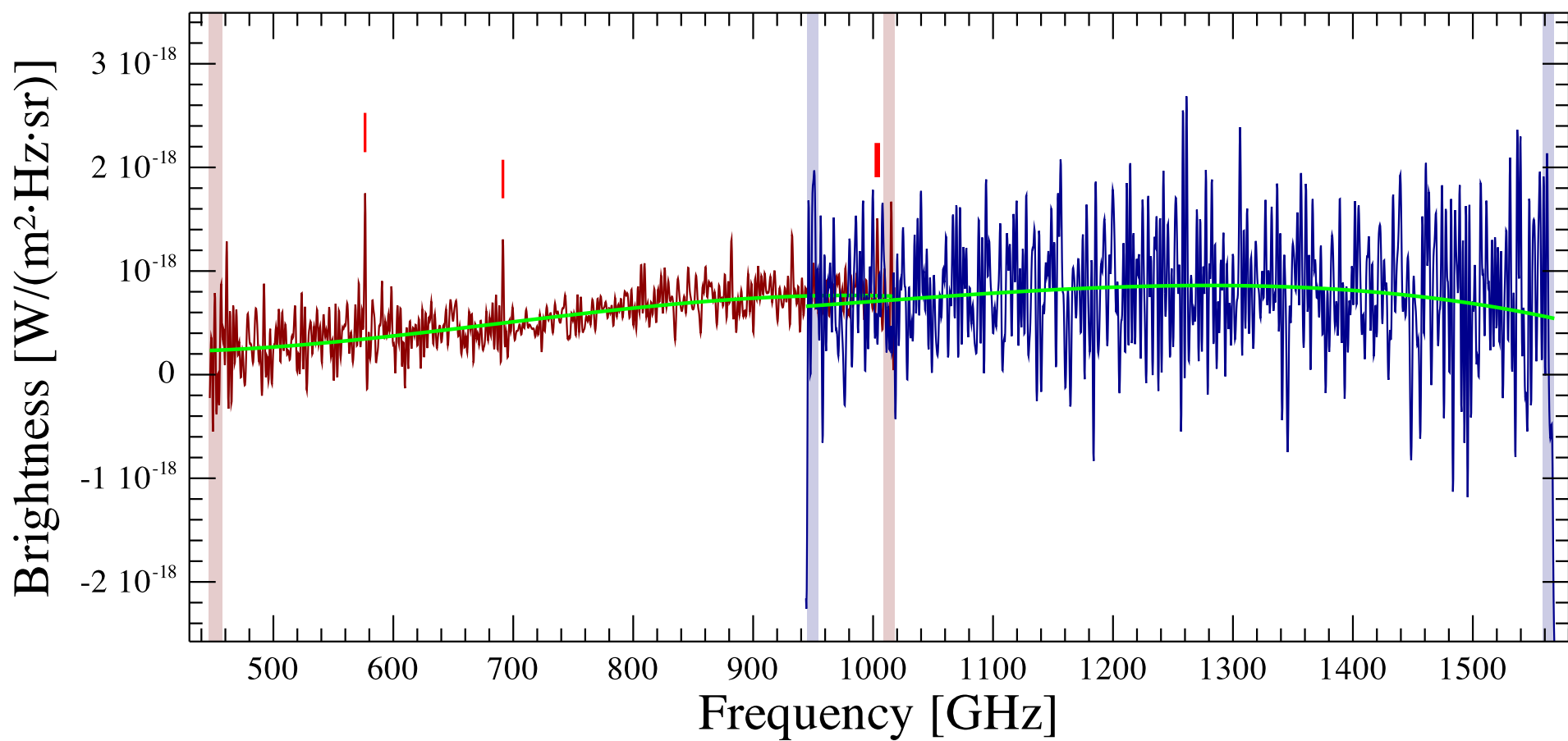
N1333-IRAS4_off Observation ID 1342213375; (3/0)
