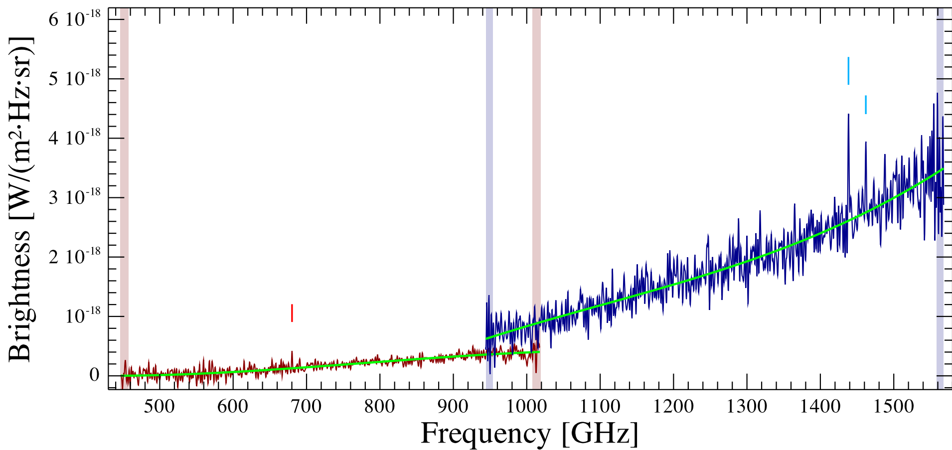
NGC6052 Observation ID 1342212347; (1/2)
