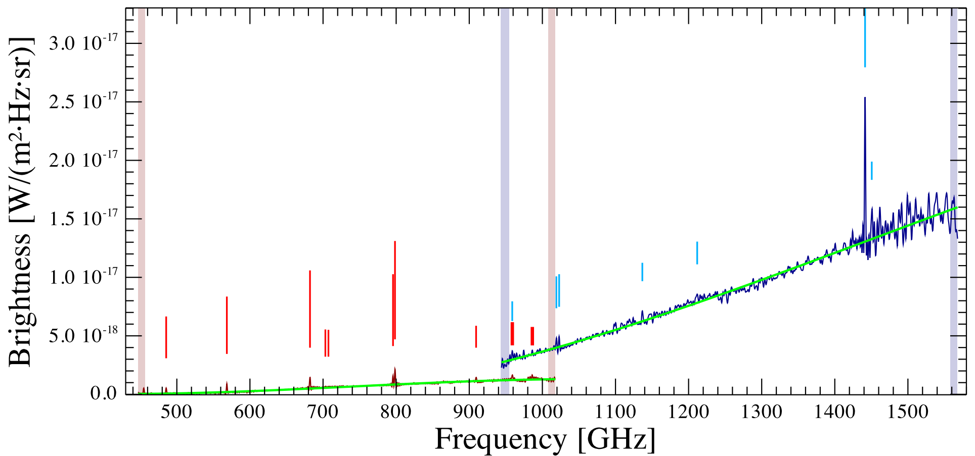
NGC5135 Observation ID 1342212344; (10/7)
