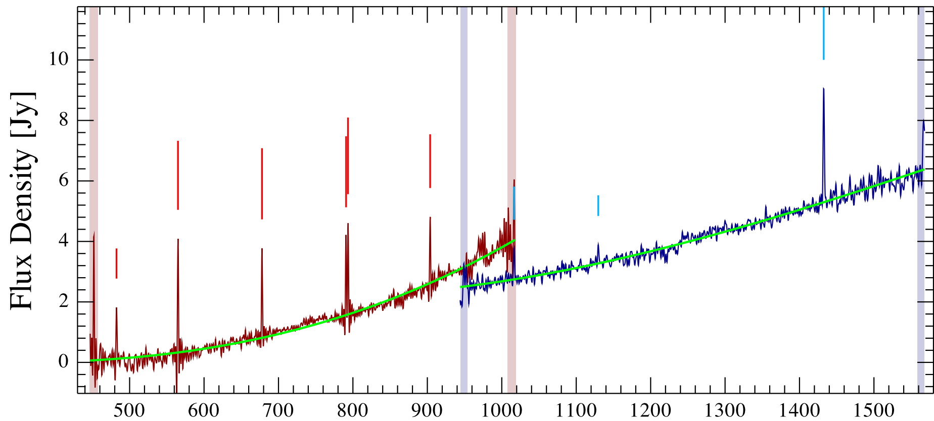
IC1623 Observation ID 1342212314; (6/3)
