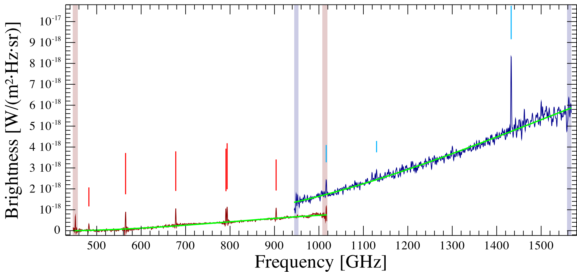
IC1623 Observation ID 1342212314; (6/3)
