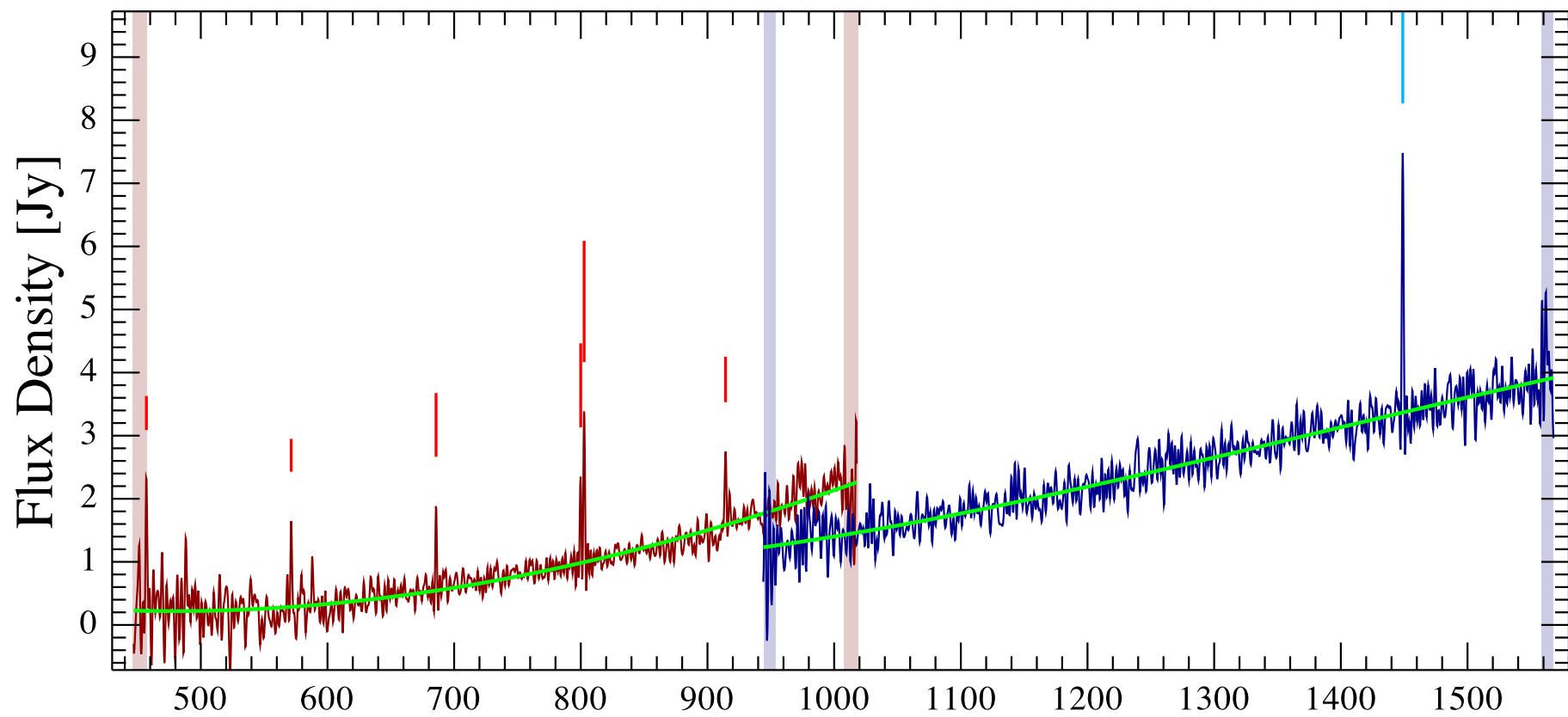
NGC4388 Observation ID 1342210849; (4/1)
