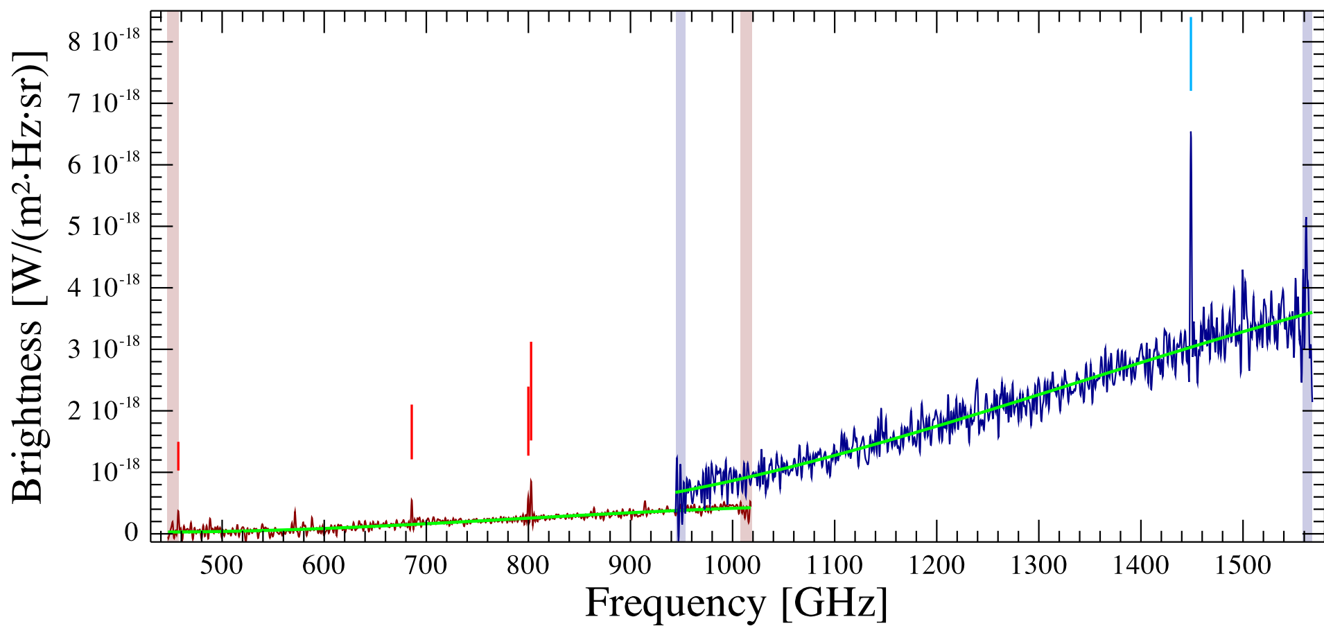
NGC4388 Observation ID 1342210849; (4/1)
