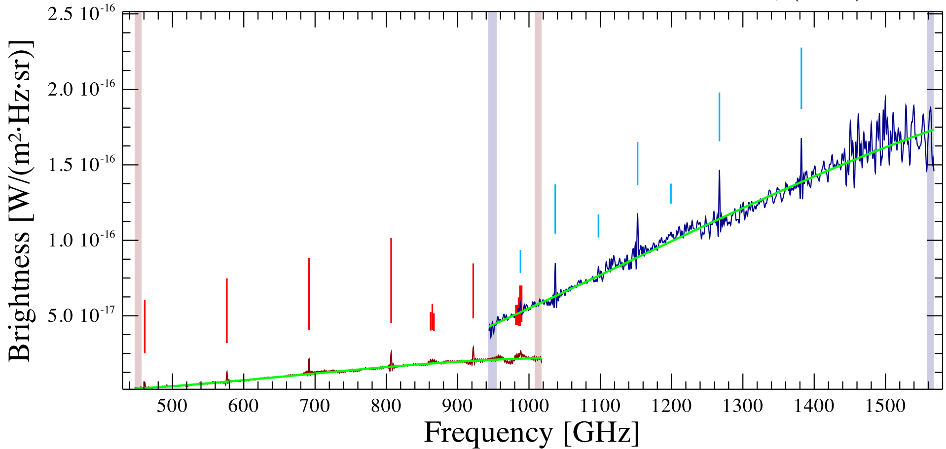
NGC_7129_IRS Observation ID 1342209857; (14/7)
