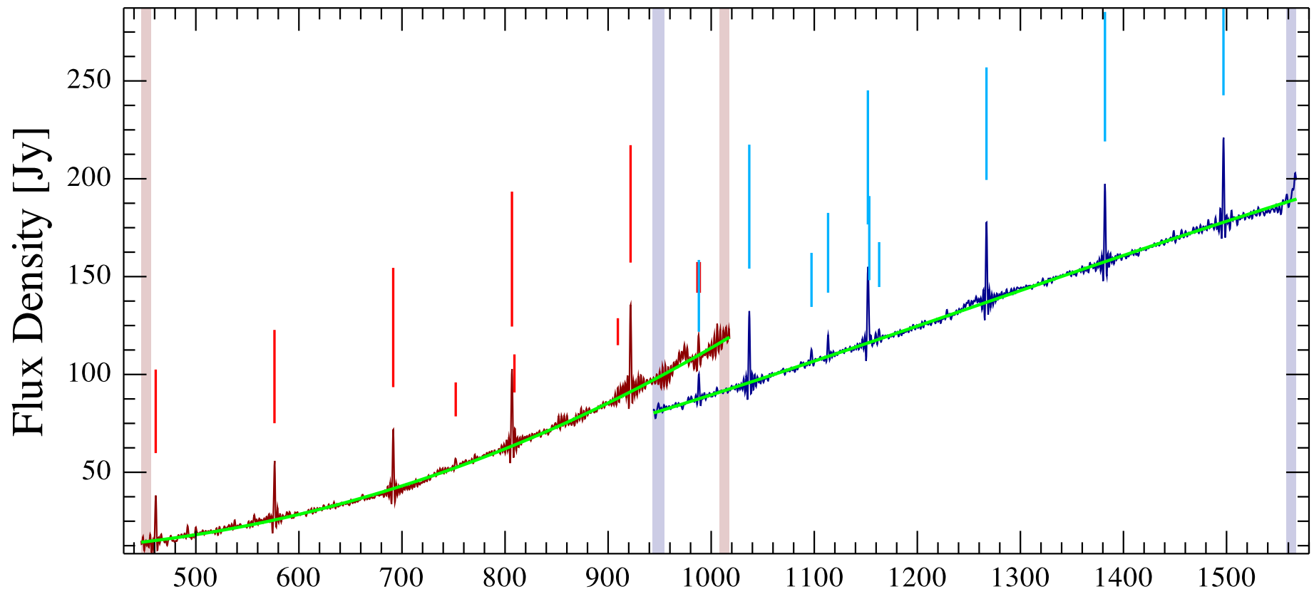
NGC_7129_IRS Observation ID 1342209857; (14/7)
