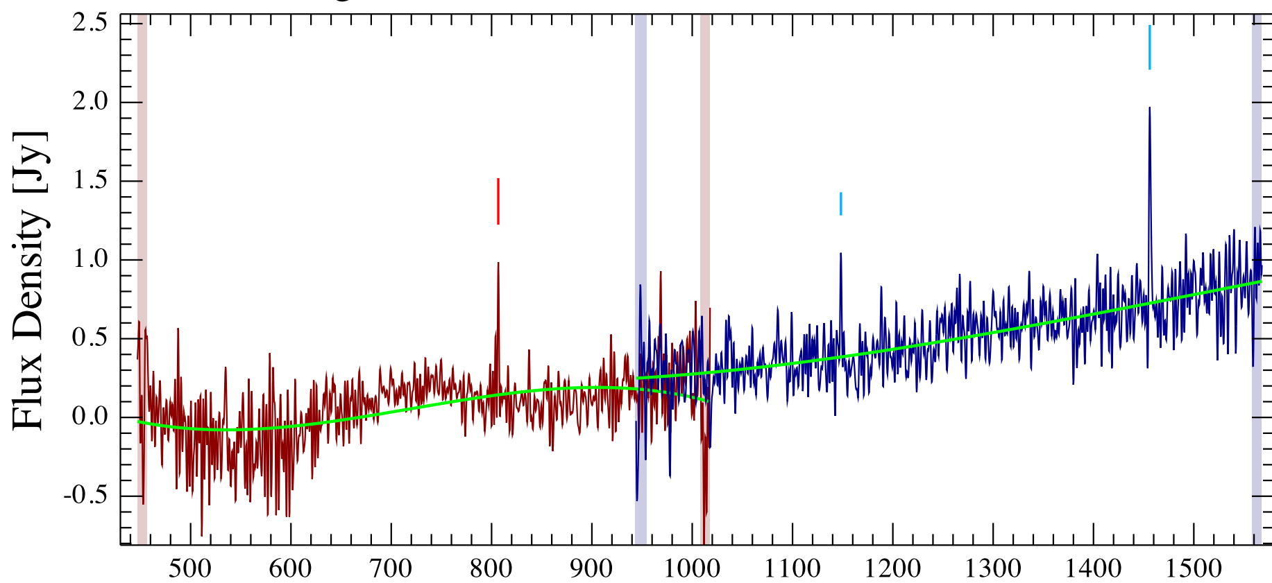
ngc4151 Observation ID 1342209852; (1/2)
