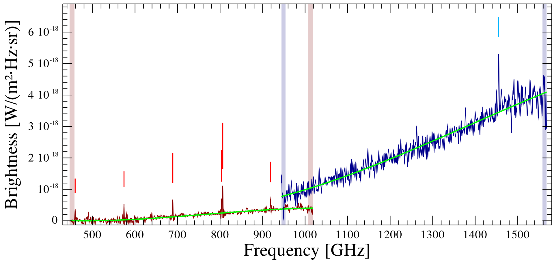
NGC3227 Observation ID 1342209281; (6/1)
