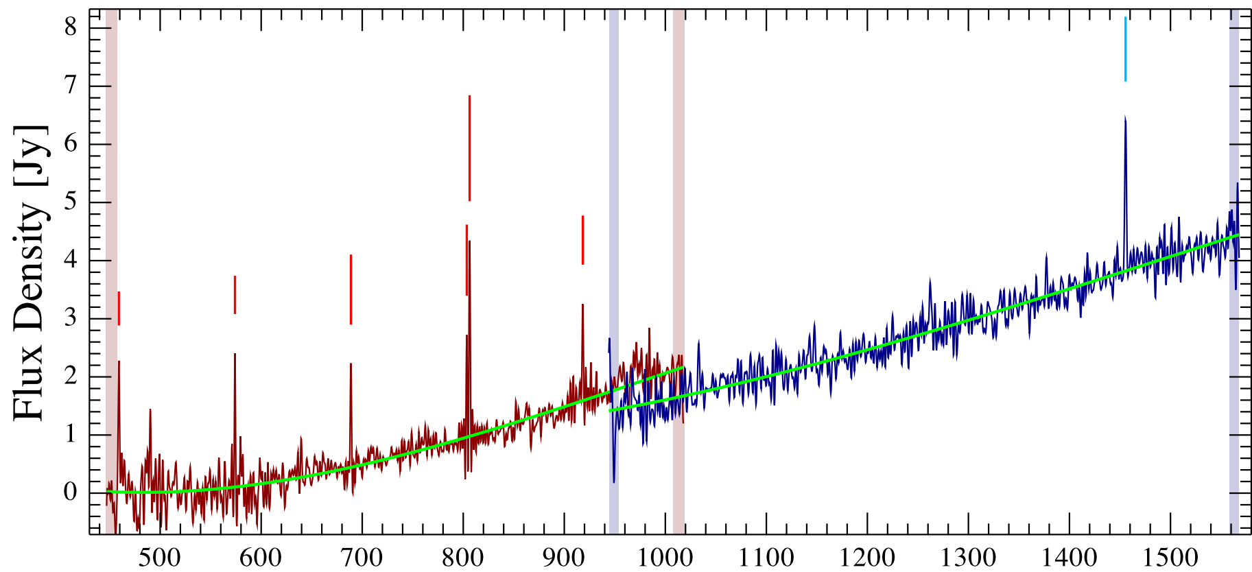
NGC3227 Observation ID 1342209281; (6/1)
