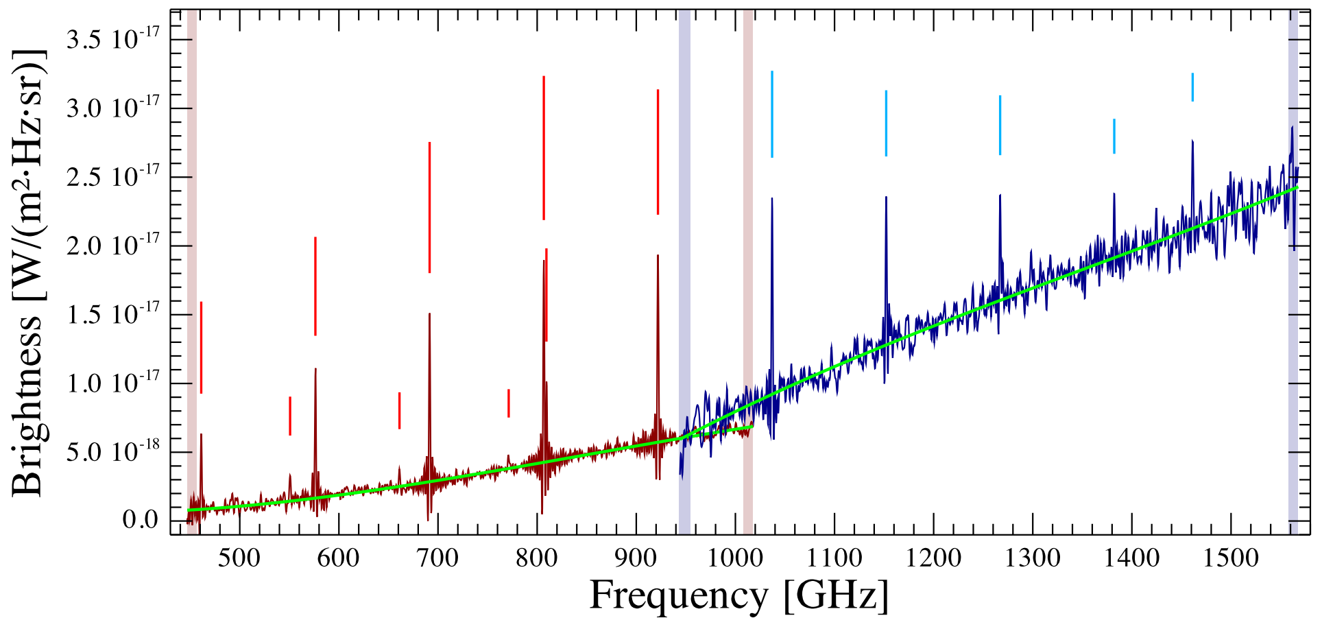
02570+6028 Observation ID 1342204930; (9/5)
