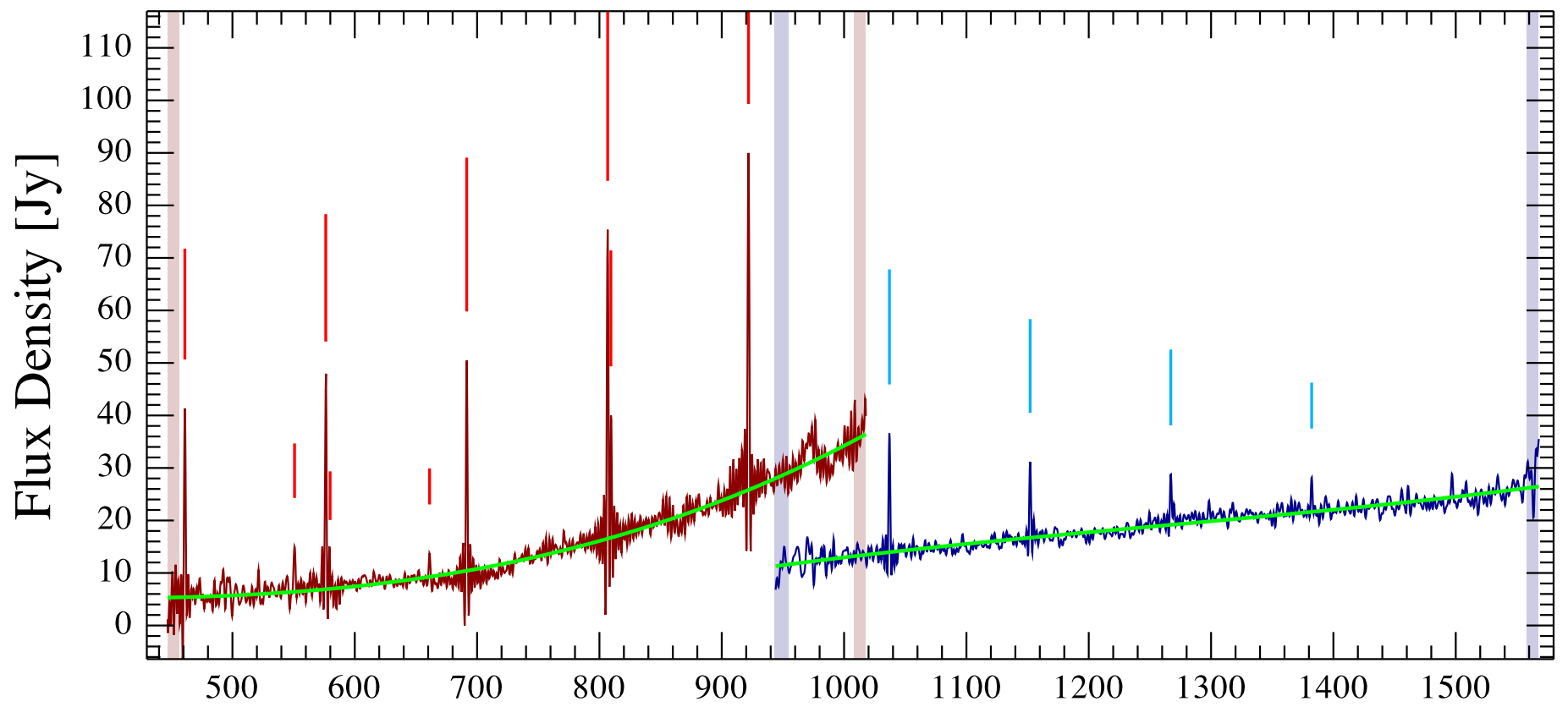
02570+6028 Observation ID 1342204930; (9/5)
