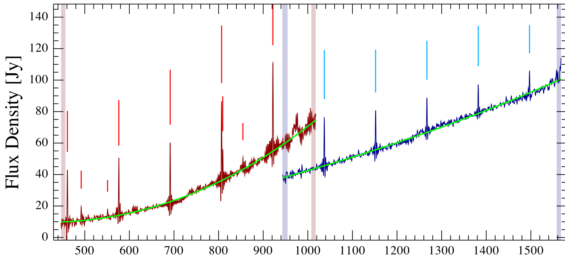
IRAS06006+3015 Observation ID 1342204924; (8/6)
