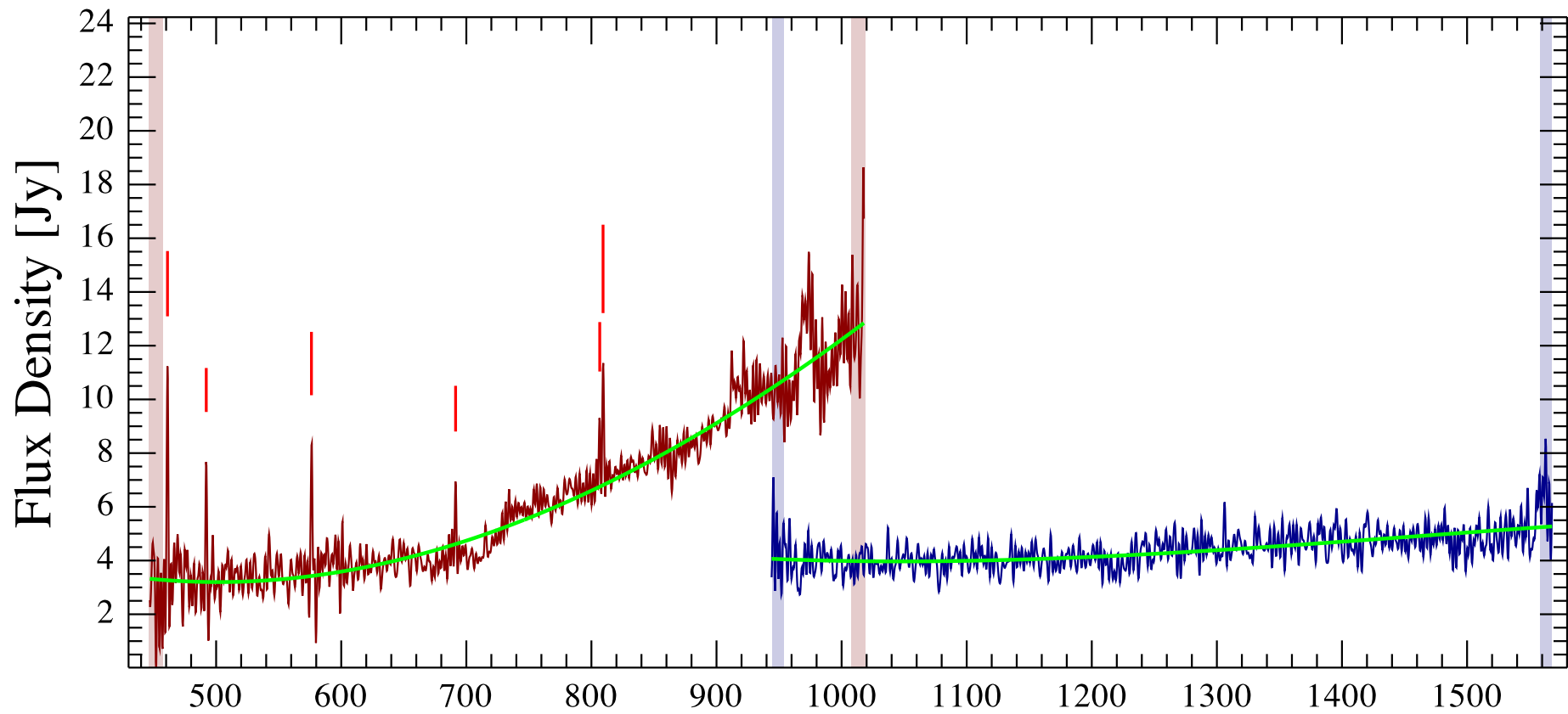
s241off Observation ID 1342204923; (7/0)
