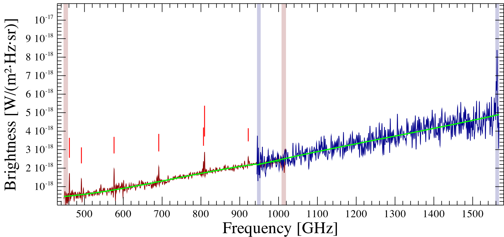
s241off Observation ID 1342204923; (7/0)
