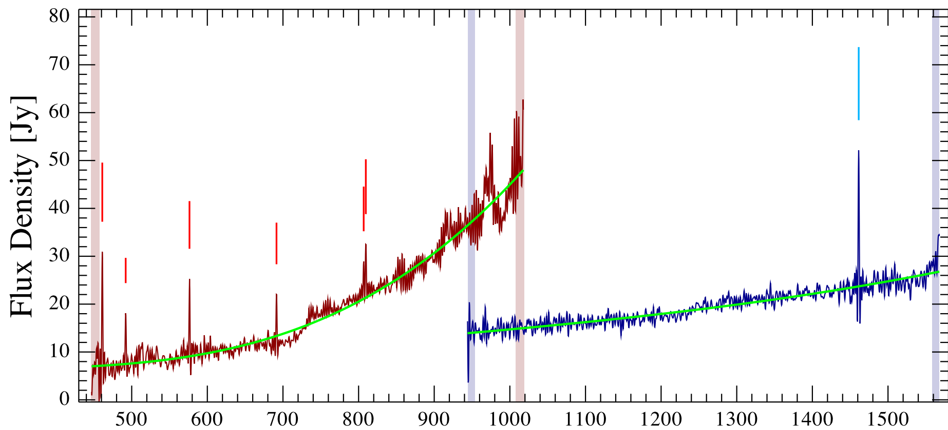
rcw82irs4 Observation ID 1342204908; (6/1)
