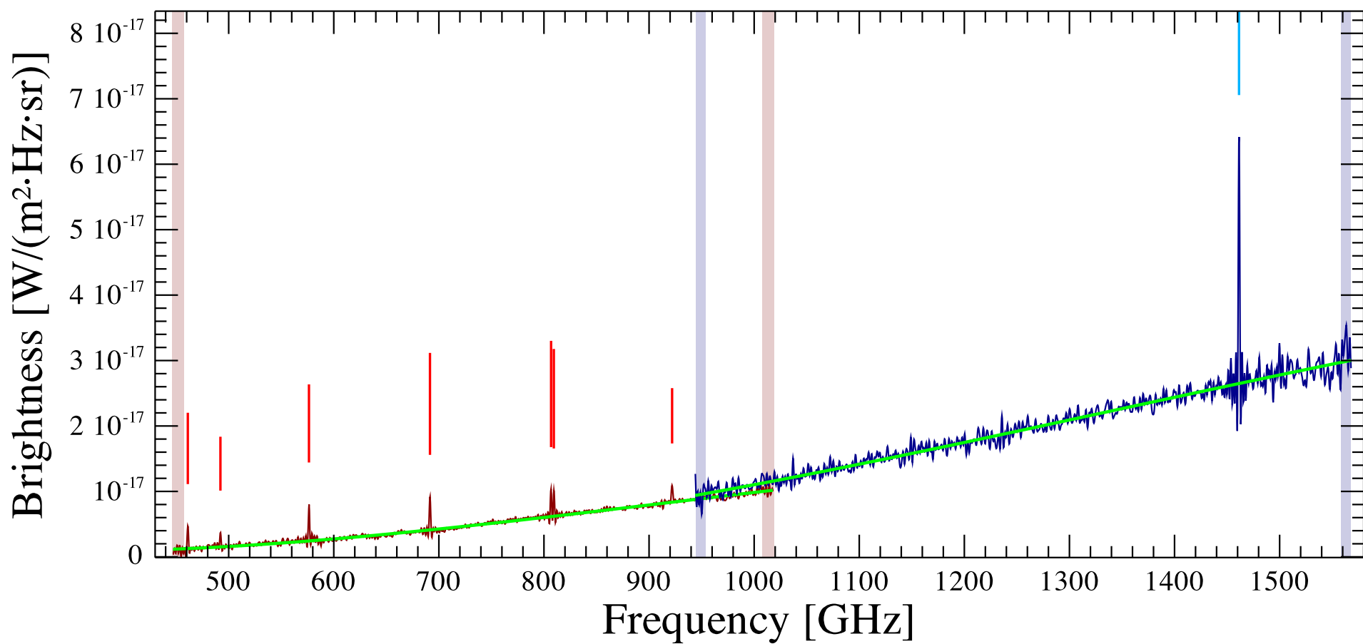
rcw82irs3 Observation ID 1342204907; (7/1)
