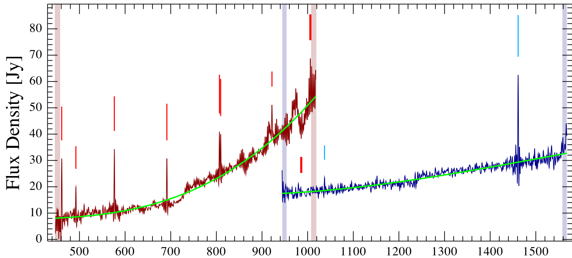
rcw82irs3 Observation ID 1342204907; (7/1)
