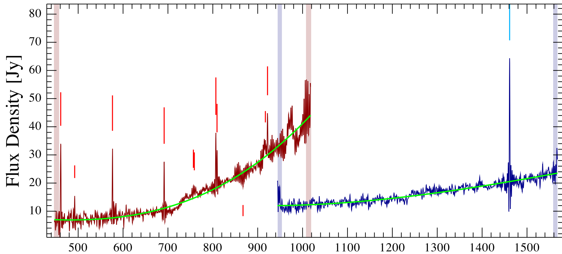
rcw82irs2 Observation ID 1342204903; (7/1)
