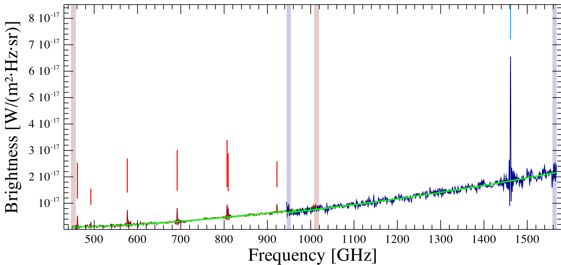
rcw82irs2 Observation ID 1342204903; (7/1)
