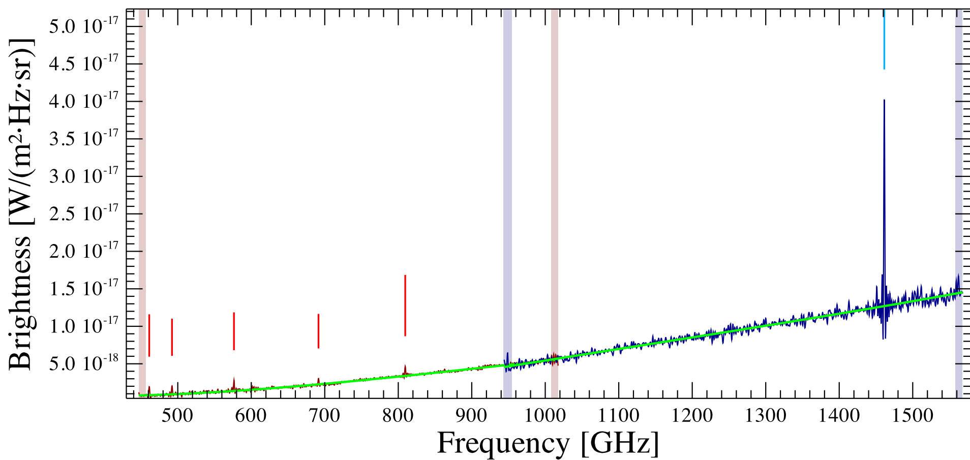
rcw82off2 Observation ID 1342204901; (5/1)
