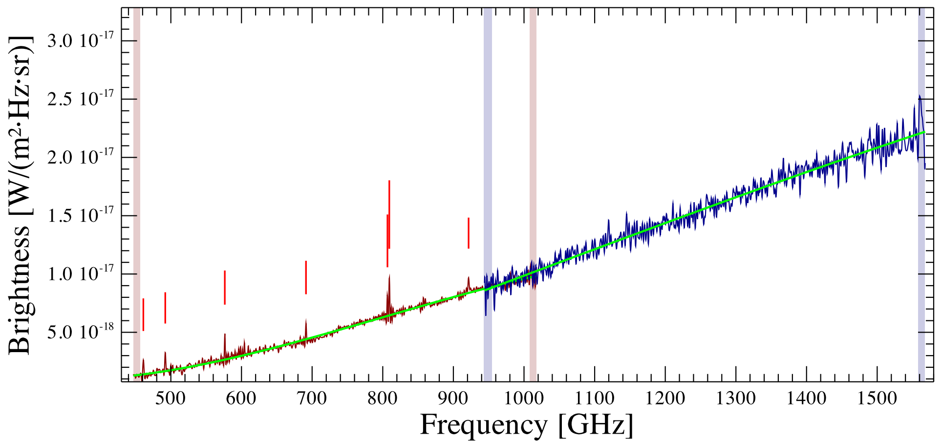
EL29_off Observation ID 1342204897; (7/0)
