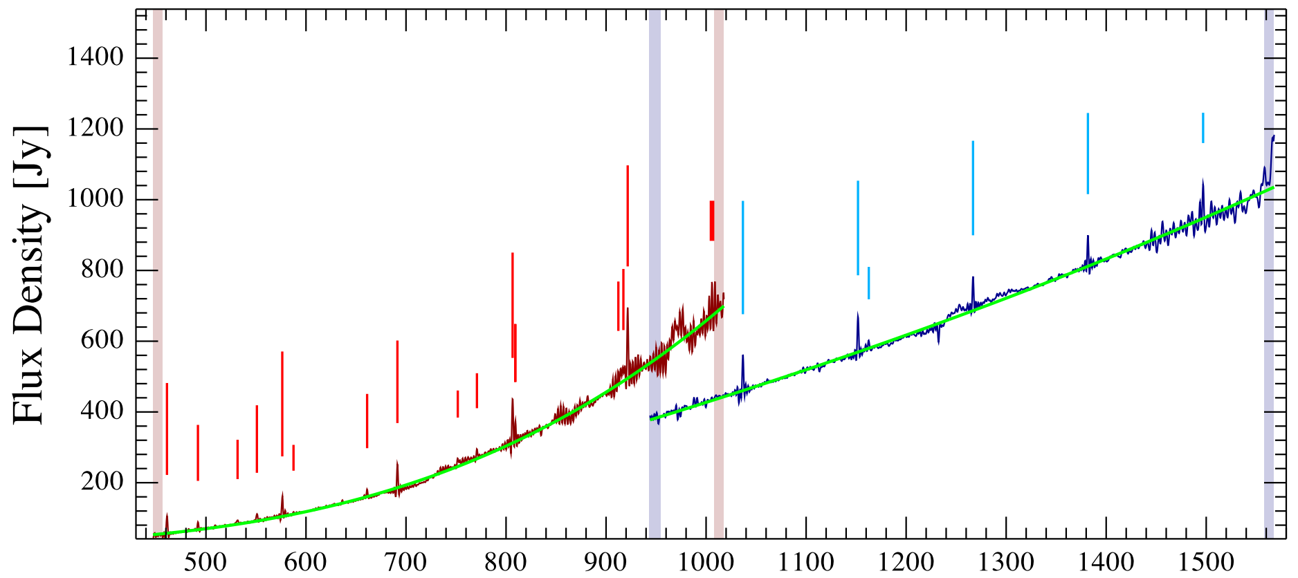
IRAS_18089 Observation ID 1342204879; (20/4)
