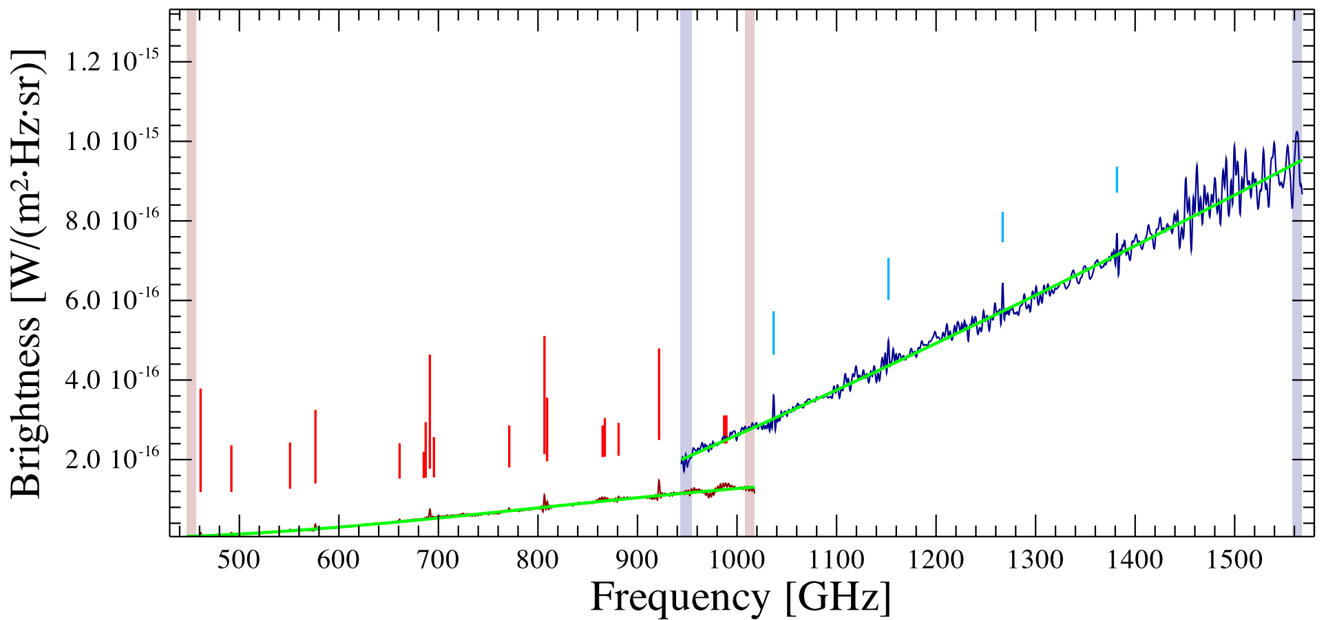
IRAS_18089 Observation ID 1342204879; (20/4)
