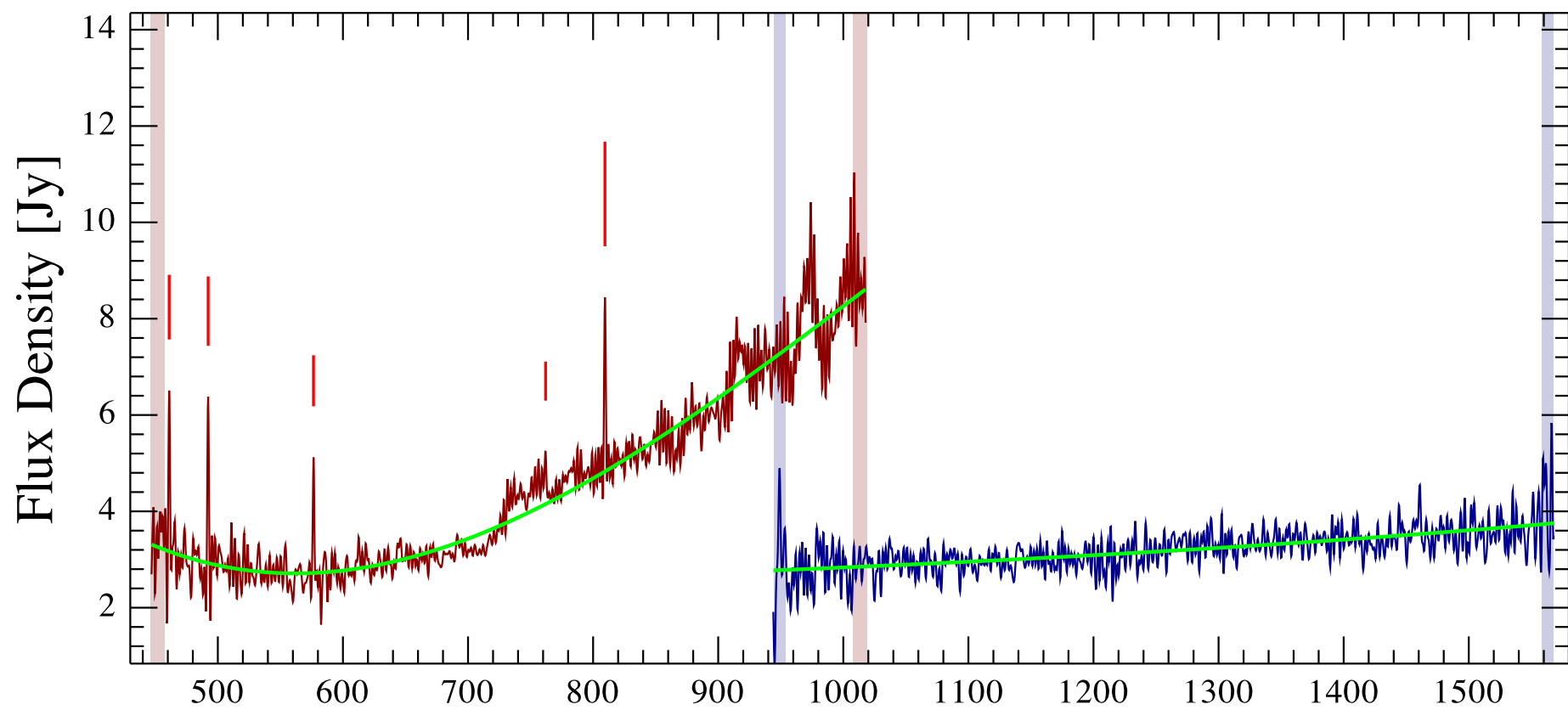
CasA FTS NW-1 Observation ID 1342204033; (4/1)
