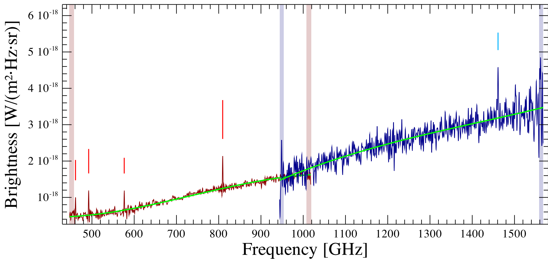
CasA FTS NW-1 Observation ID 1342204033; (4/1)
