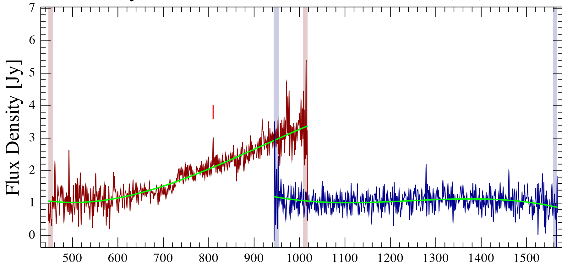
Tycho SP1 Observation ID 1342204032; (2/0)
