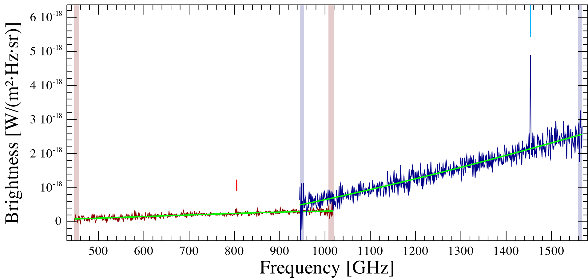
NGC1056 Observation ID 1342204024; (1/1)
