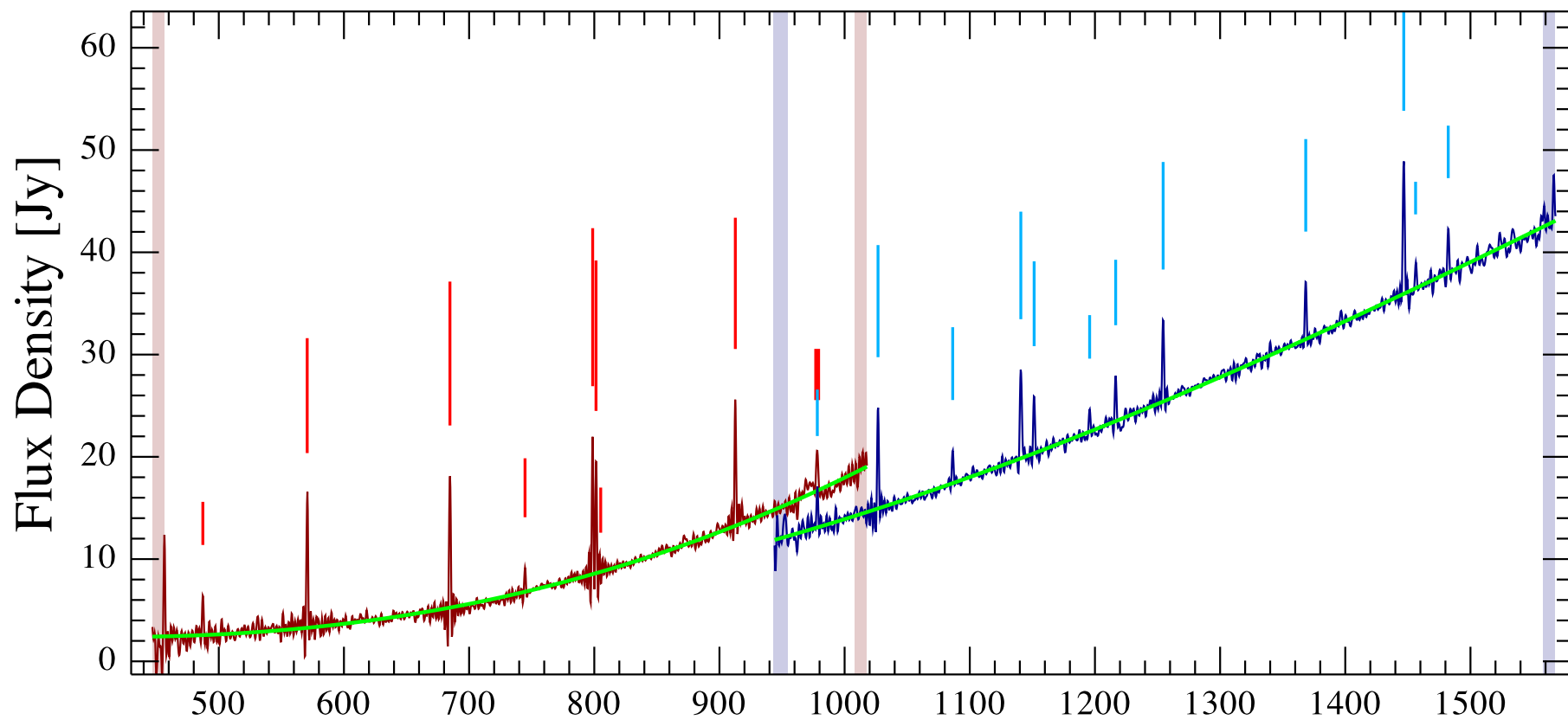
ESO 173-G015 Observation ID 1342202268; (8/12)
