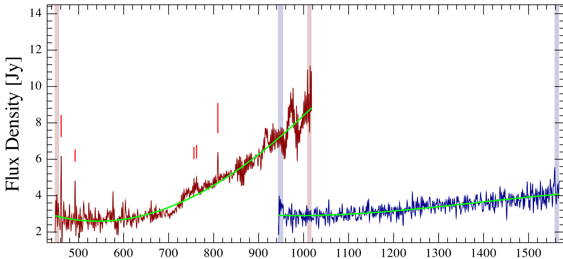
Cas A FTS Centre-1 Observation ID 1342202265; (4/0)
