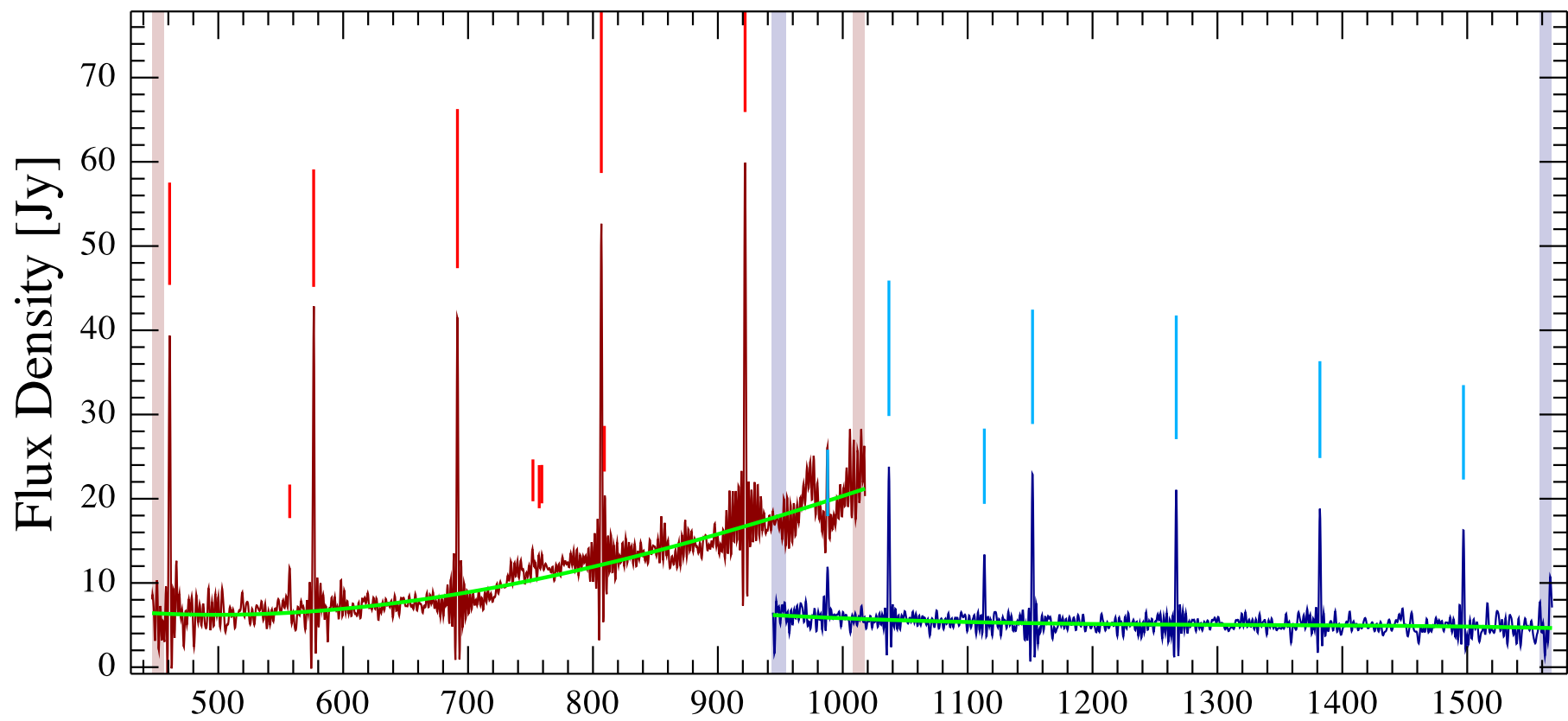
L1448-B2 Observation ID 1342202264; (9/7)
