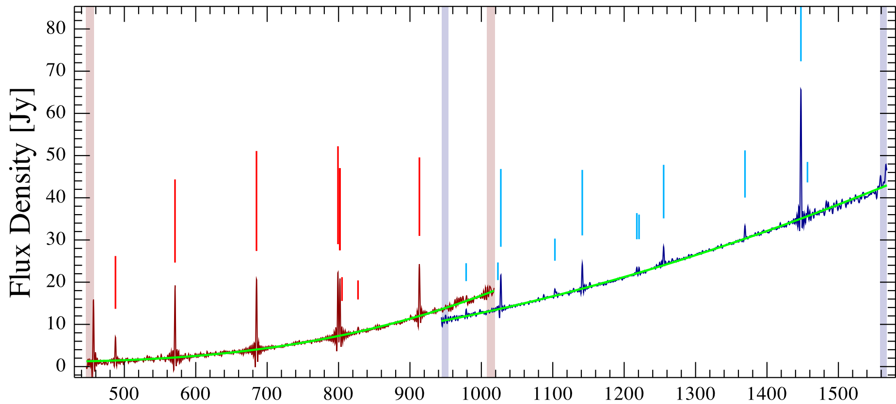
NGC3256 Observation ID 1342201201; (8/7)
