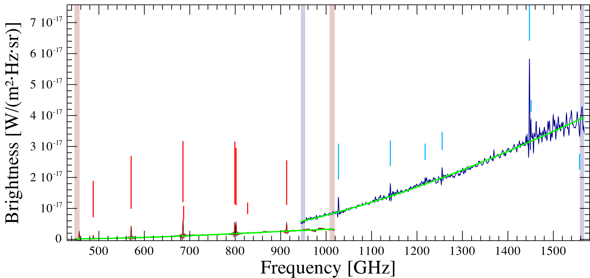
NGC3256 Observation ID 1342201201; (8/7)
